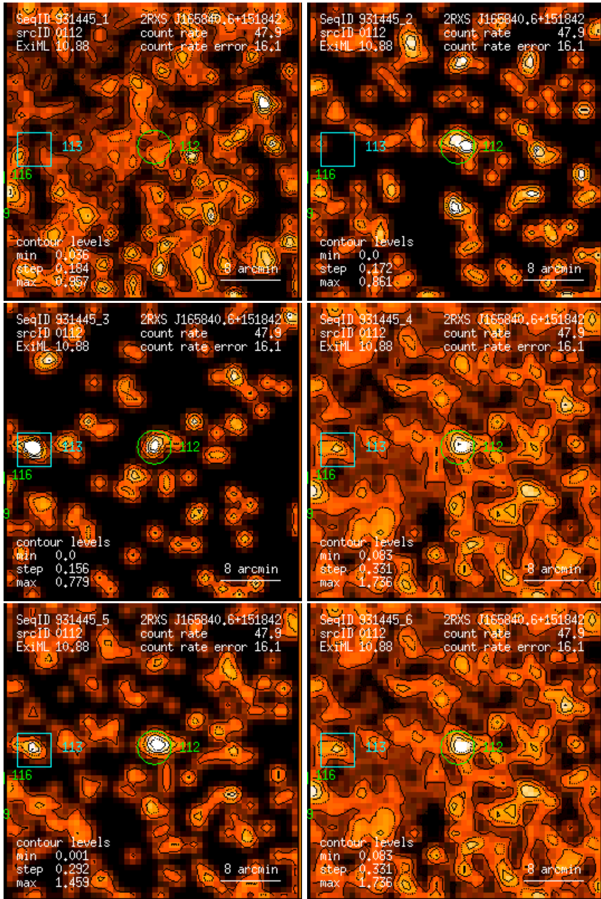
Figure 112: RASS 931445: detection 0112: band rate images, Gaussian filter: (1) PSPC channels 11 – 41, (2) 52 – 90, (3) 91 – 201, (4) 11 – 235, (5) 52 – 201, (6) 11 – 201. Broad band rates in counts/ks. Band rate contour levels in counts/ks/arcmin 2 .
