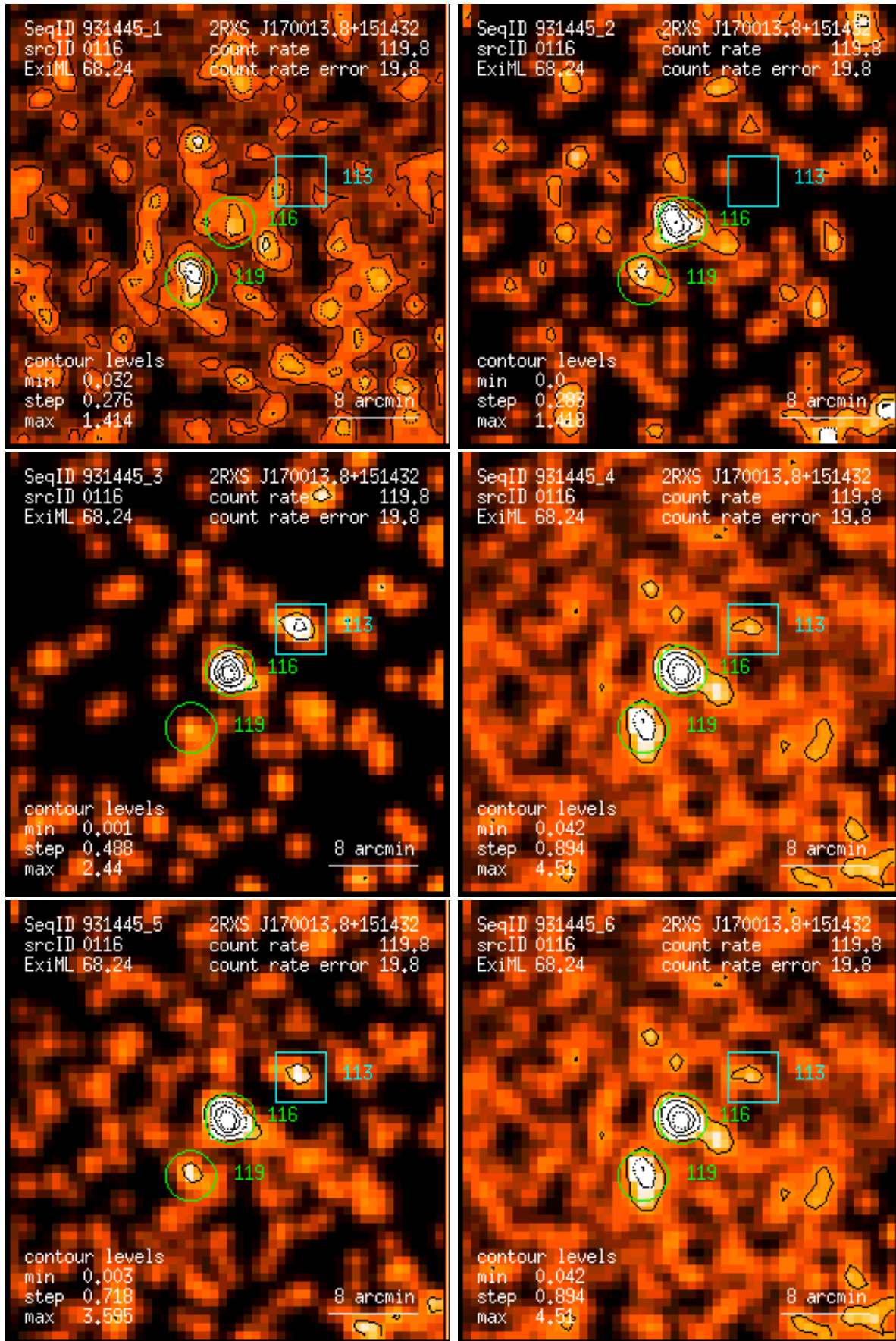
Figure 116: RASS 931445: detection 0116: band rate images, Gaussian filter: (1) PSPC channels 11 – 41, (2) 52 – 90, (3) 91 – 201, (4) 11 – 235, (5) 52 – 201, (6) 11 – 201. Broad band rates in counts/ks. Band rate contour levels in counts/ks/arcmin 2 .
