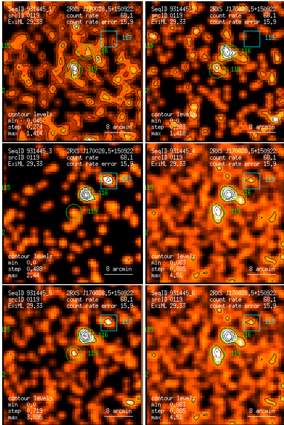
Figure 119: RASS 931445: detection 0119: band rate images, Gaussian filter: (1) PSPC channels 11 – 41, (2) 52 – 90, (3) 91 – 201, (4) 11 – 235, (5) 52 – 201, (6) 11 – 201. Broad band rates in counts/ks. Band rate contour levels in counts/ks/arcmin 2 .
