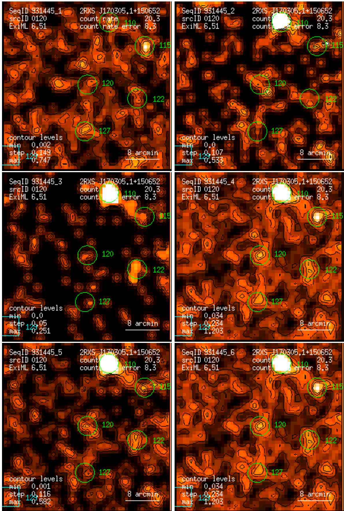
Figure 120: RASS 931445: detection 0120: band rate images, Gaussian filter: (1) PSPC channels 11 – 41, (2) 52 – 90, (3) 91 – 201, (4) 11 – 235, (5) 52 – 201, (6) 11 – 201. Broad band rates in counts/ks. Band rate contour levels in counts/ks/arcmin 2 .
