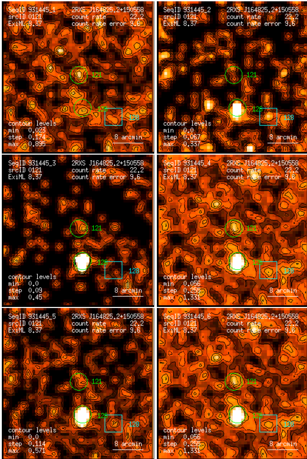
Figure 121: RASS 931445: detection 0121: band rate images, Gaussian filter: (1) PSPC channels 11 – 41, (2) 52 – 90, (3) 91 – 201, (4) 11 – 235, (5) 52 – 201, (6) 11 – 201. Broad band rates in counts/ks. Band rate contour levels in counts/ks/arcmin 2 .
