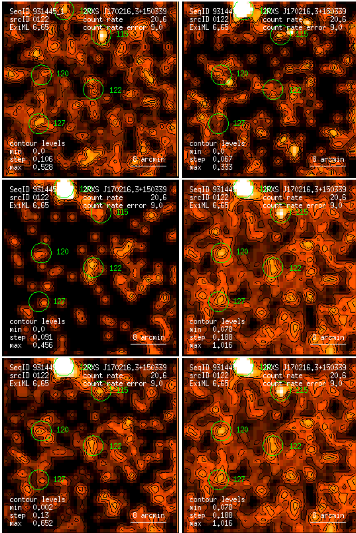
Figure 122: RASS 931445: detection 0122: band rate images, Gaussian filter: (1) PSPC channels 11 – 41, (2) 52 – 90, (3) 91 – 201, (4) 11 – 235, (5) 52 – 201, (6) 11 – 201. Broad band rates in counts/ks. Band rate contour levels in counts/ks/arcmin 2 .
