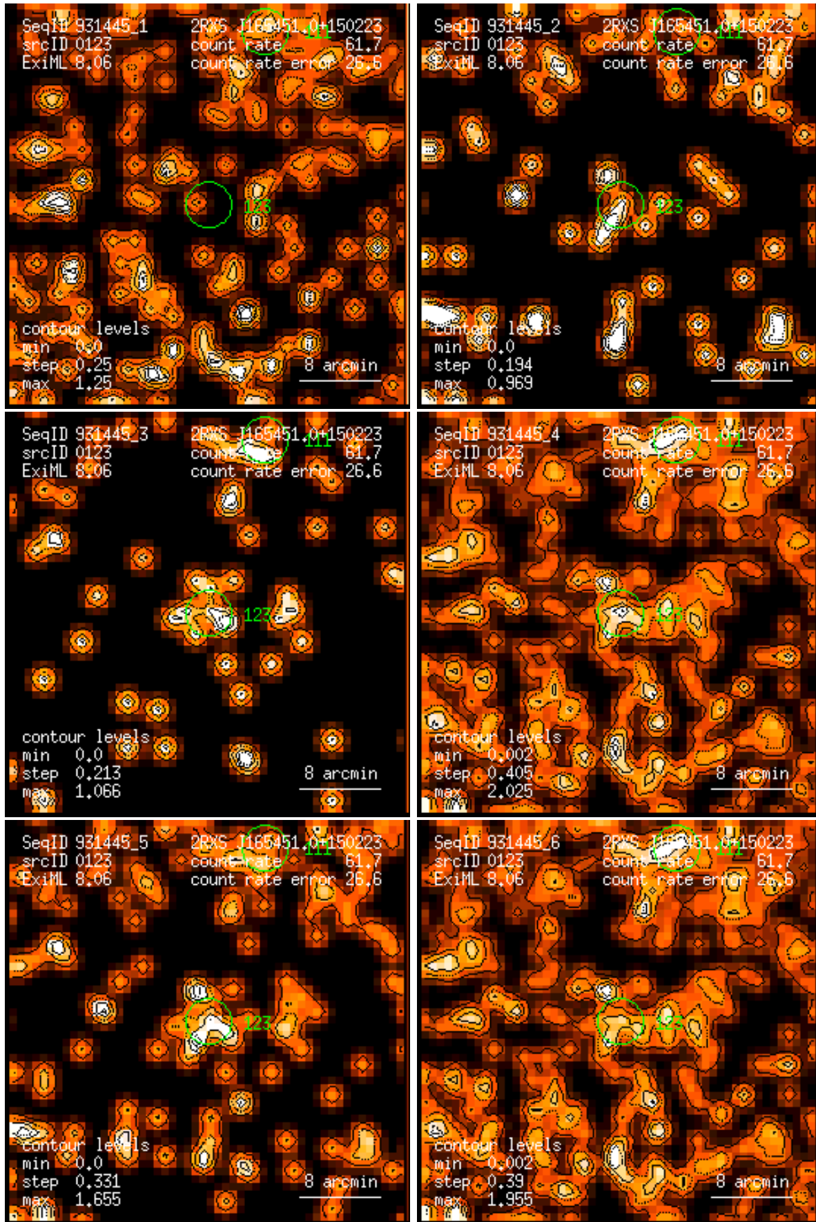
Figure 123: RASS 931445: detection 0123: band rate images, Gaussian filter: (1) PSPC channels 11 – 41, (2) 52 – 90, (3) 91 – 201, (4) 11 – 235, (5) 52 – 201, (6) 11 – 201. Broad band rates in counts/ks. Band rate contour levels in counts/ks/arcmin 2 .
