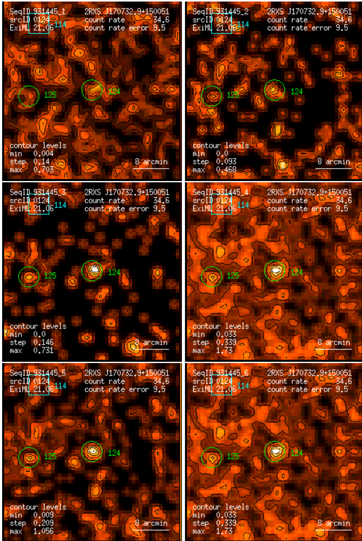
Figure 124: RASS 931445: detection 0124: band rate images, Gaussian filter: (1) PSPC channels 11 – 41, (2) 52 – 90, (3) 91 – 201, (4) 11 – 235, (5) 52 – 201, (6) 11 – 201. Broad band rates in counts/ks. Band rate contour levels in counts/ks/arcmin 2 .
