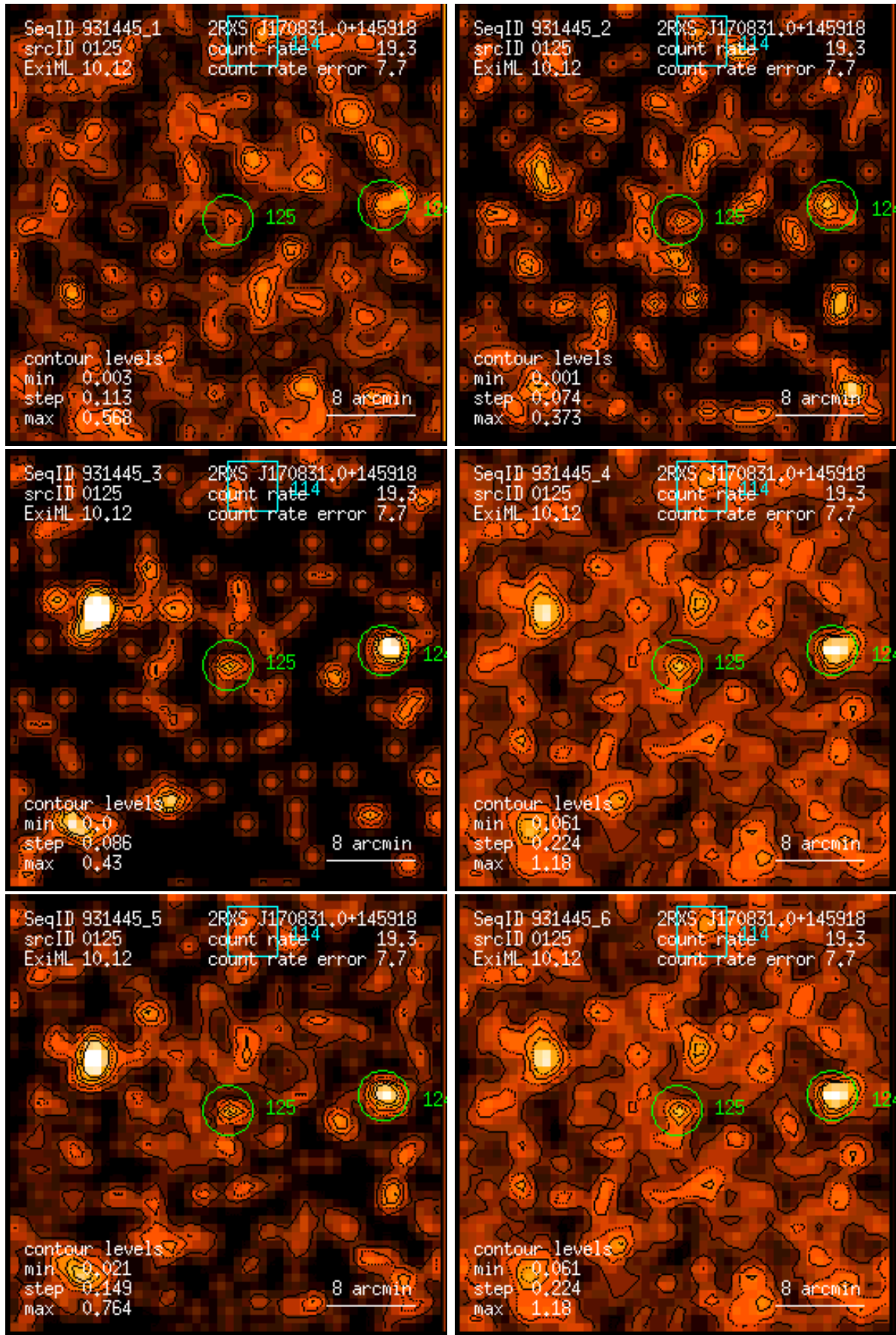
Figure 125: RASS 931445: detection 0125: band rate images, Gaussian filter: (1) PSPC channels 11 – 41, (2) 52 – 90, (3) 91 – 201, (4) 11 – 235, (5) 52 – 201, (6) 11 – 201. Broad band rates in counts/ks. Band rate contour levels in counts/ks/arcmin 2 .
