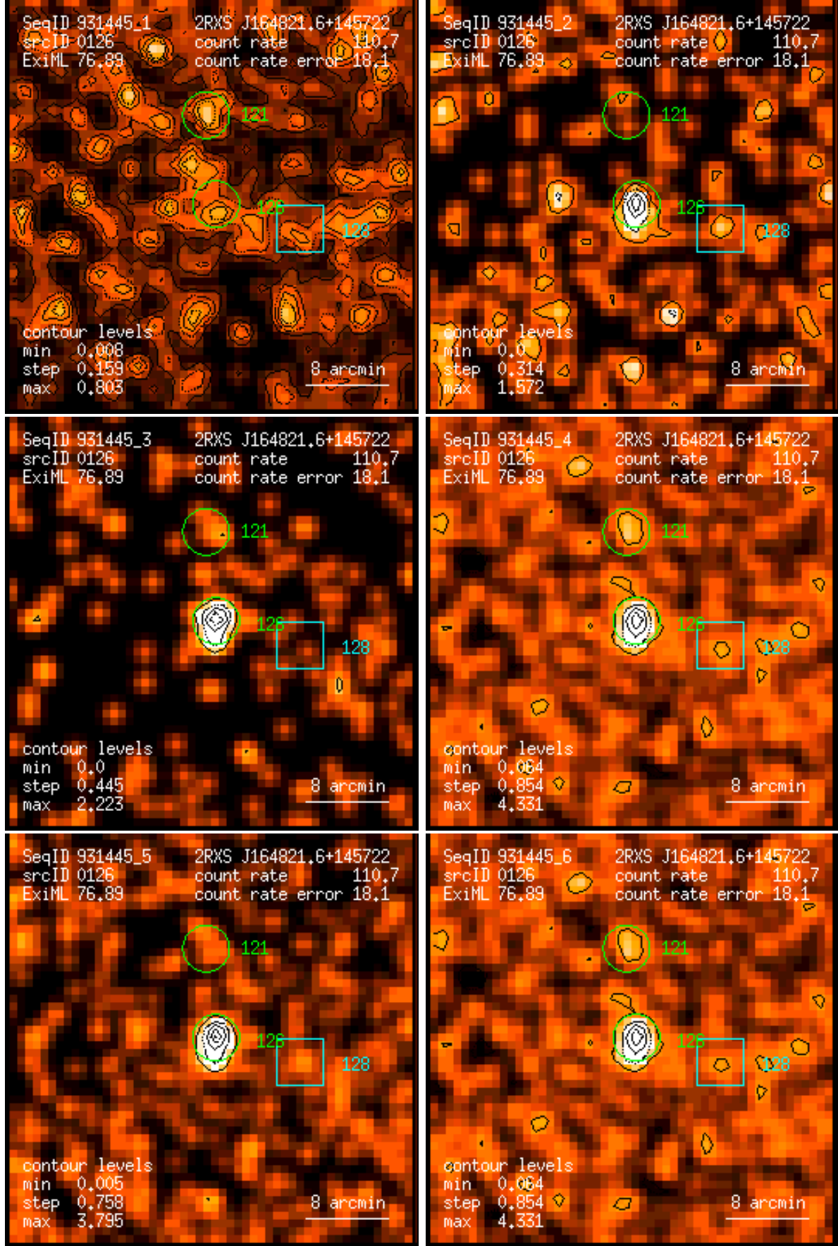
Figure 126: RASS 931445: detection 0126: band rate images, Gaussian filter: (1) PSPC channels 11 – 41, (2) 52 – 90, (3) 91 – 201, (4) 11 – 235, (5) 52 – 201, (6) 11 – 201. Broad band rates in counts/ks. Band rate contour levels in counts/ks/arcmin 2 .
