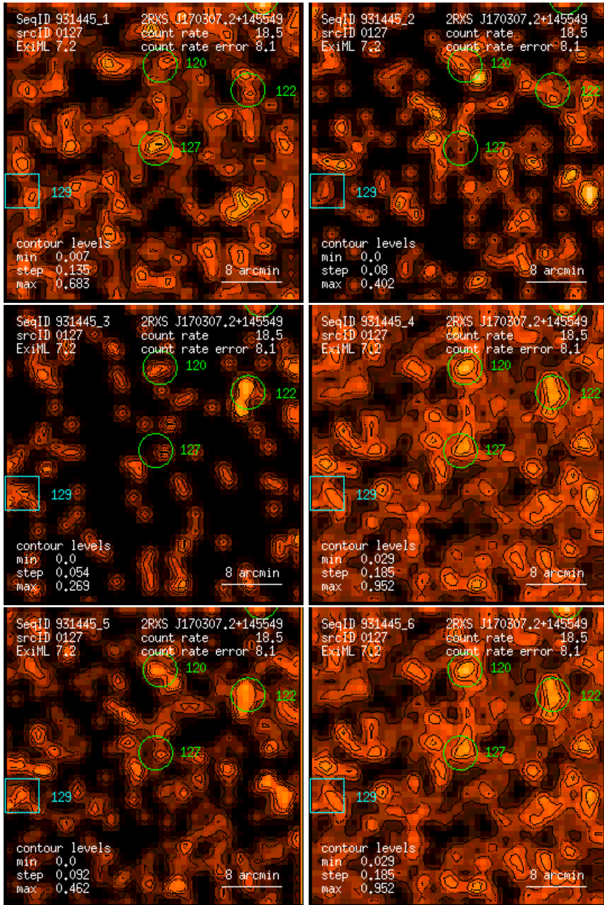
Figure 127: RASS 931445: detection 0127: band rate images, Gaussian filter: (1) PSPC channels 11 – 41, (2) 52 – 90, (3) 91 – 201, (4) 11 – 235, (5) 52 – 201, (6) 11 – 201. Broad band rates in counts/ks. Band rate contour levels in counts/ks/arcmin 2 .
