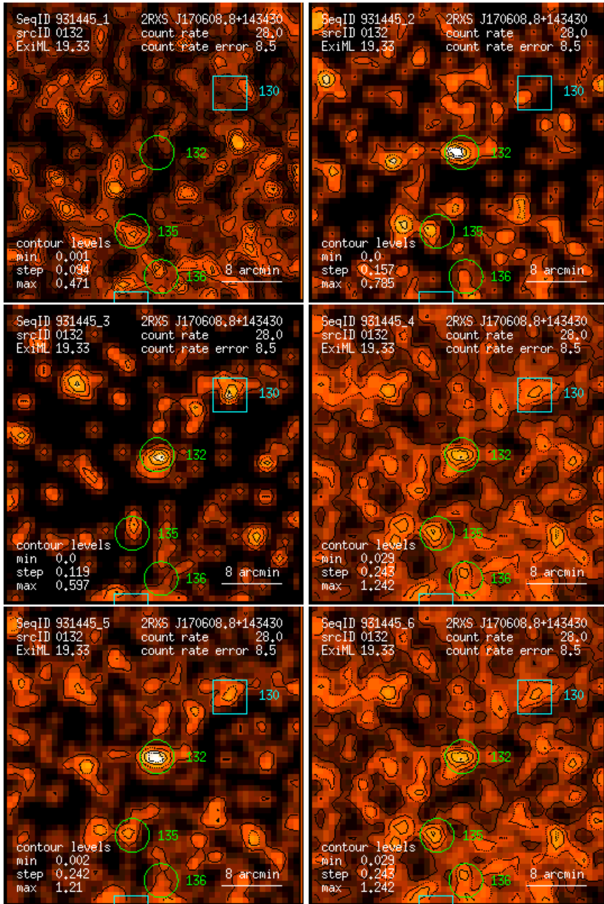
Figure 132: RASS 931445: detection 0132: band rate images, Gaussian filter: (1) PSPC channels 11 – 41, (2) 52 – 90, (3) 91 – 201, (4) 11 – 235, (5) 52 – 201, (6) 11 – 201. Broad band rates in counts/ks. Band rate contour levels in counts/ks/arcmin 2 .
