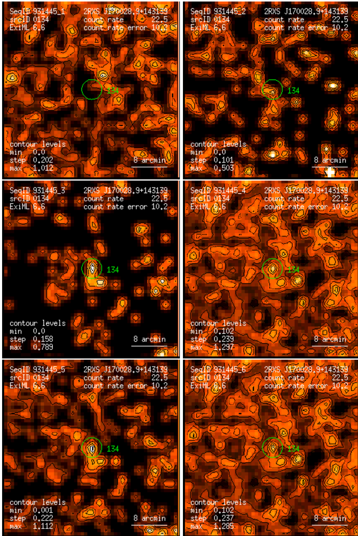
Figure 134: RASS 931445: detection 0134: band rate images, Gaussian filter: (1) PSPC channels 11 – 41, (2) 52 – 90, (3) 91 – 201, (4) 11 – 235, (5) 52 – 201, (6) 11 – 201. Broad band rates in counts/ks. Band rate contour levels in counts/ks/arcmin 2 .
