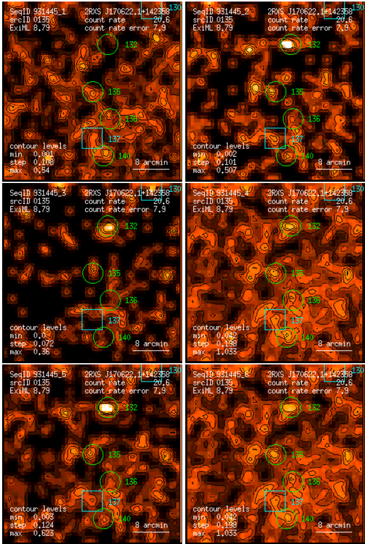
Figure 135: RASS 931445: detection 0135: band rate images, Gaussian filter: (1) PSPC channels 11 – 41, (2) 52 – 90, (3) 91 – 201, (4) 11 – 235, (5) 52 – 201, (6) 11 – 201. Broad band rates in counts/ks. Band rate contour levels in counts/ks/arcmin 2 .
