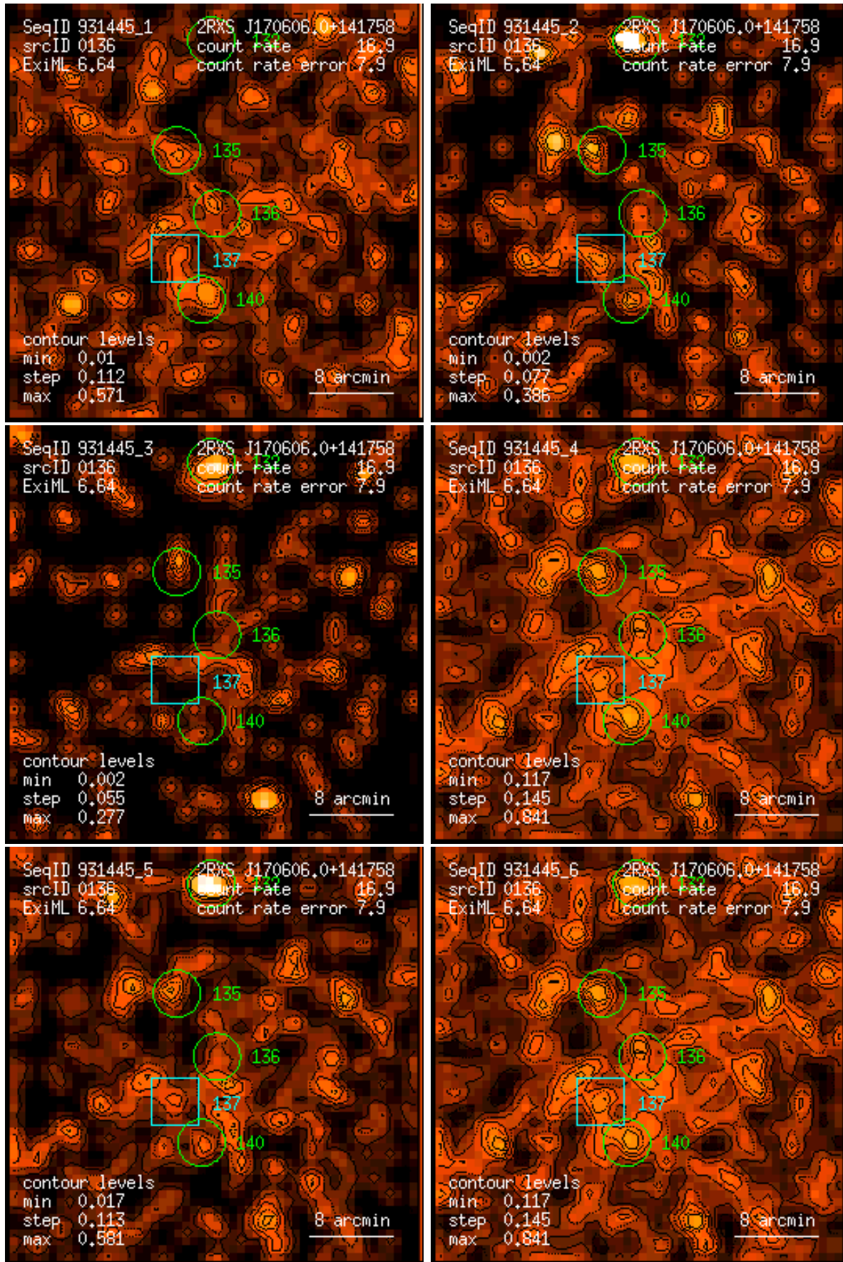
Figure 136: RASS 931445: detection 0136: band rate images, Gaussian filter: (1) PSPC channels 11 – 41, (2) 52 – 90, (3) 91 – 201, (4) 11 – 235, (5) 52 – 201, (6) 11 – 201. Broad band rates in counts/ks. Band rate contour levels in counts/ks/arcmin 2 .
