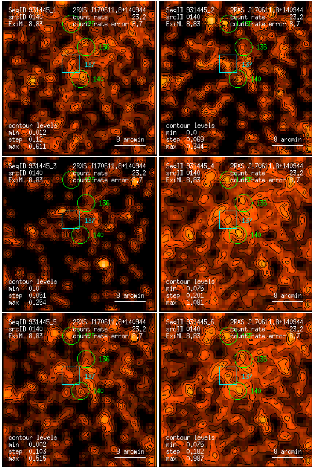
Figure 140: RASS 931445: detection 0140: band rate images, Gaussian filter: (1) PSPC channels 11 – 41, (2) 52 – 90, (3) 91 – 201, (4) 11 – 235, (5) 52 – 201, (6) 11 – 201. Broad band rates in counts/ks. Band rate contour levels in counts/ks/arcmin 2 .
