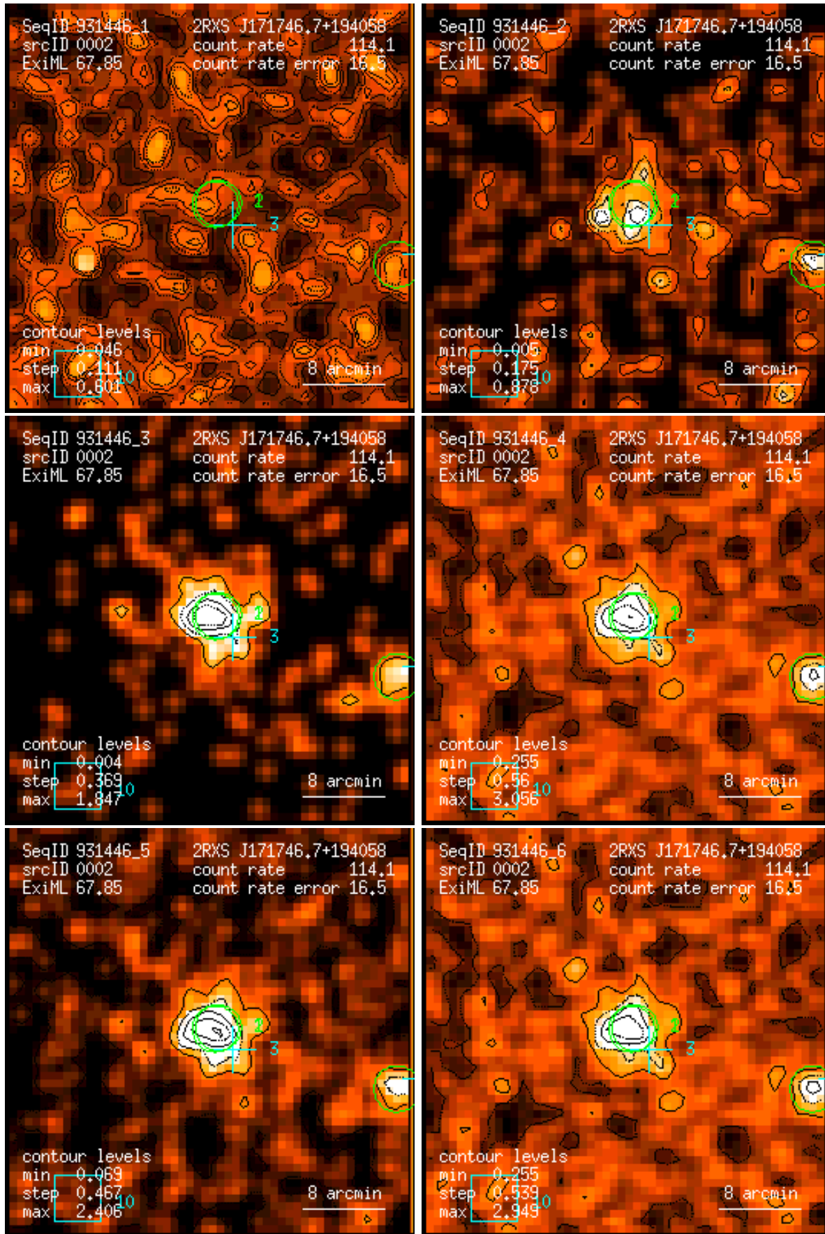
Figure 2: RASS 931446: detection 0002: band rate images, Gaussian filter: (1) PSPC channels 11 – 41, (2) 52 – 90, (3) 91 – 201, (4) 11 – 235, (5) 52 – 201, (6) 11 – 201. Broad band rates in counts/ks. Band rate contour levels in counts/ks/arcmin 2 .
