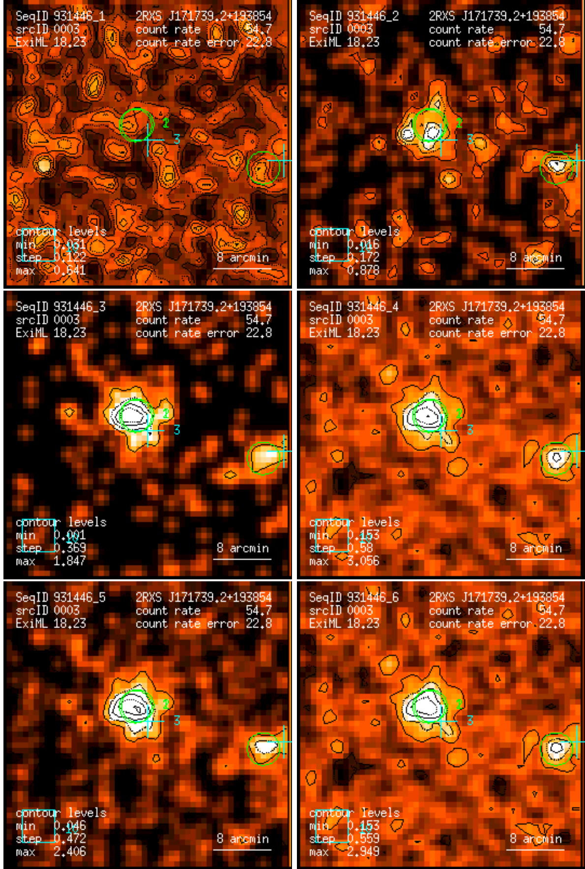
Figure 3: RASS 931446: detection 0003: band rate images, Gaussian filter: (1) PSPC channels 11 – 41, (2) 52 – 90, (3) 91 – 201, (4) 11 – 235, (5) 52 – 201, (6) 11 – 201. Broad band rates in counts/ks. Band rate contour levels in counts/ks/arcmin 2 .
