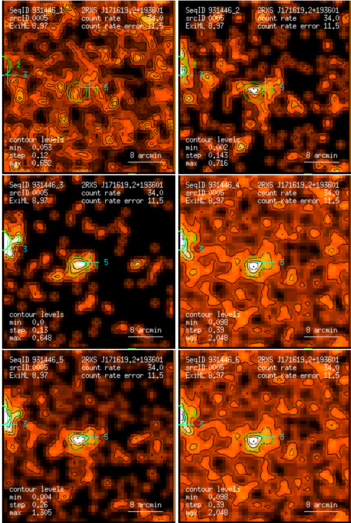
Figure 5: RASS 931446: detection 0005: band rate images, Gaussian filter: (1) PSPC channels 11 – 41, (2) 52 – 90, (3) 91 – 201, (4) 11 – 235, (5) 52 – 201, (6) 11 – 201. Broad band rates in counts/ks. Band rate contour levels in counts/ks/arcmin 2 .
