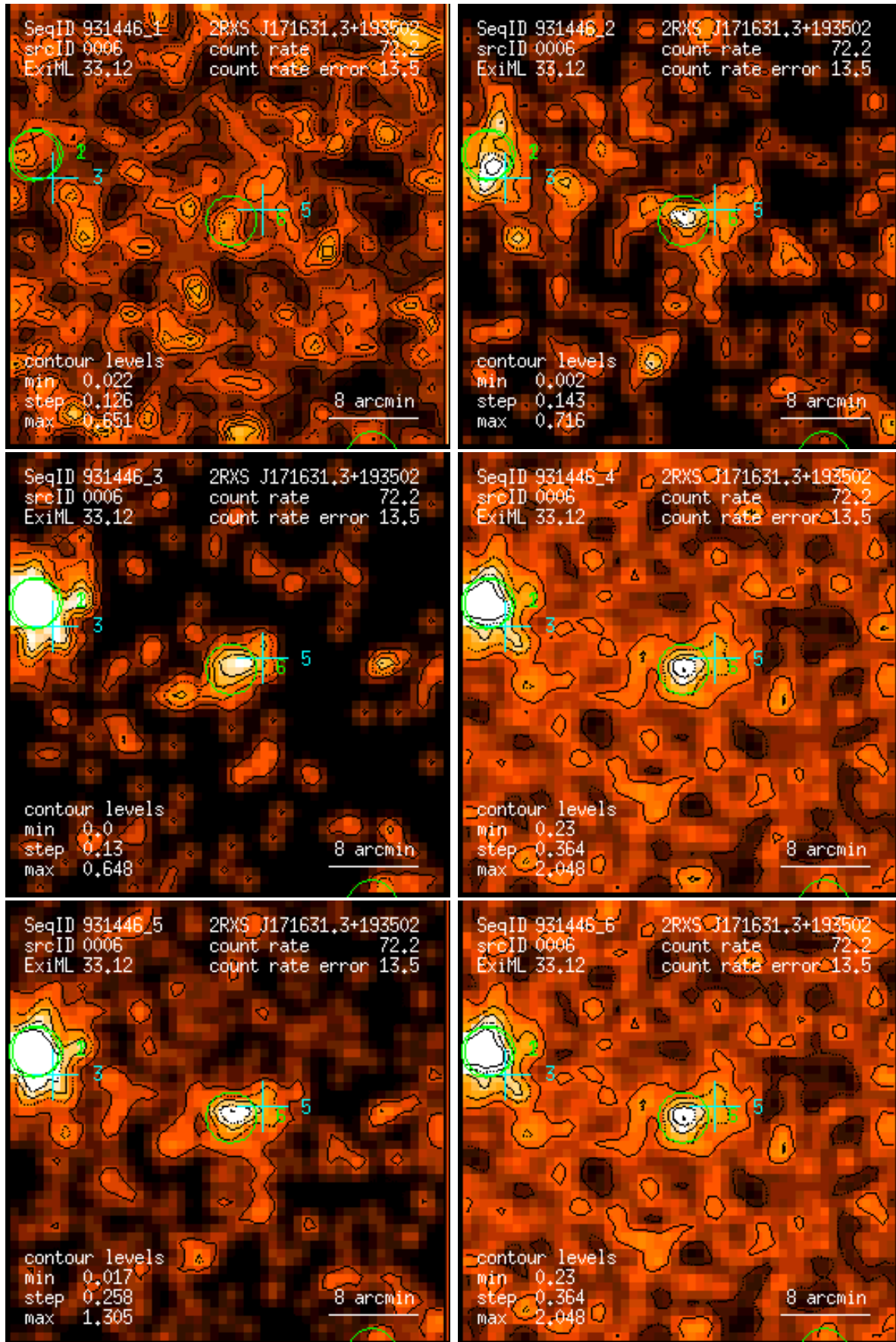
Figure 6: RASS 931446: detection 0006: band rate images, Gaussian filter: (1) PSPC channels 11 – 41, (2) 52 – 90, (3) 91 – 201, (4) 11 – 235, (5) 52 – 201, (6) 11 – 201. Broad band rates in counts/ks. Band rate contour levels in counts/ks/arcmin 2 .
