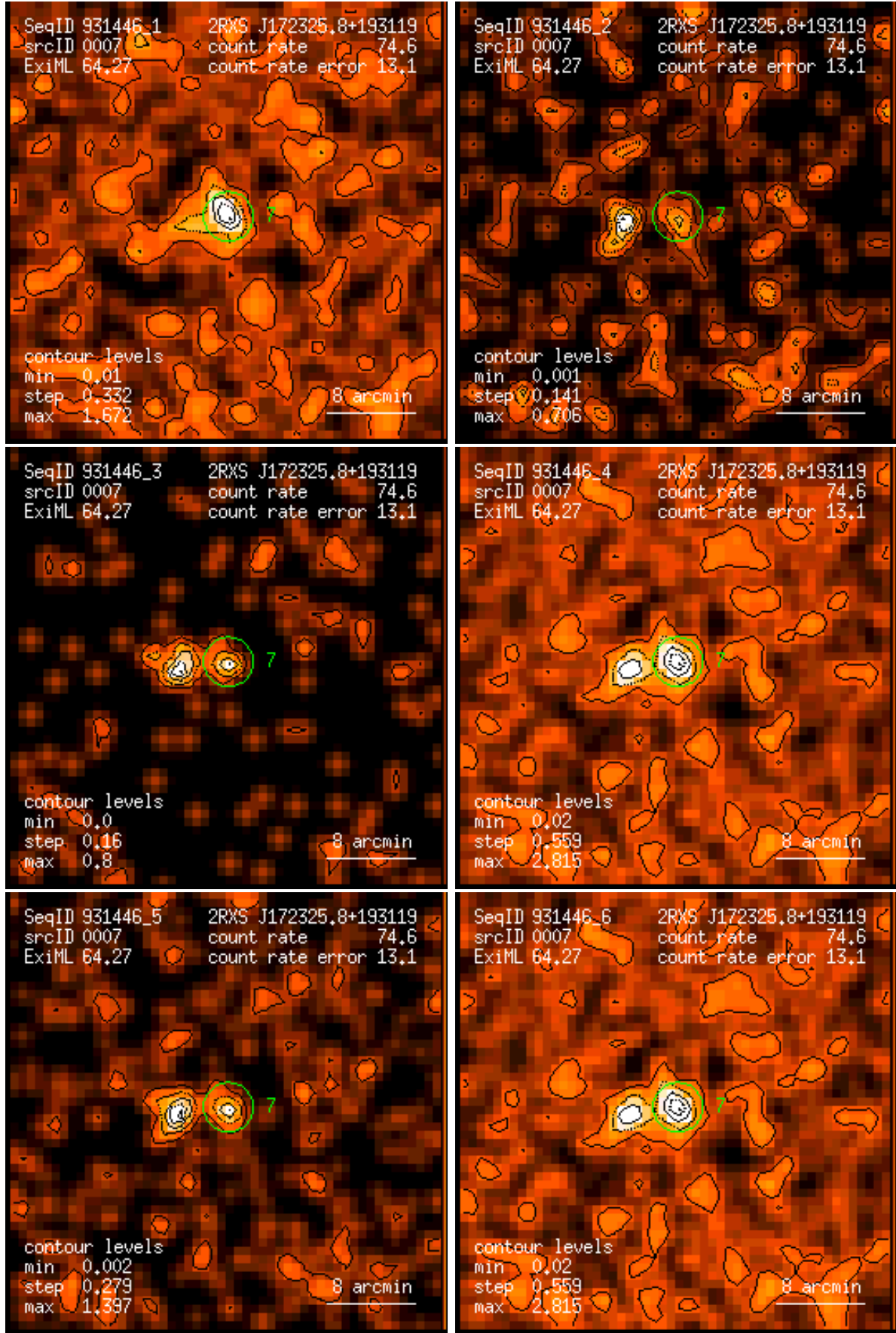
Figure 7: RASS 931446: detection 0007: band rate images, Gaussian filter: (1) PSPC channels 11 – 41, (2) 52 – 90, (3) 91 – 201, (4) 11 – 235, (5) 52 – 201, (6) 11 – 201. Broad band rates in counts/ks. Band rate contour levels in counts/ks/arcmin 2 .
