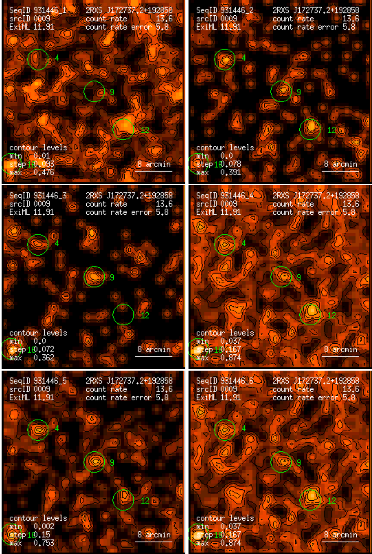
Figure 9: RASS 931446: detection 0009: band rate images, Gaussian filter: (1) PSPC channels 11 – 41, (2) 52 – 90, (3) 91 – 201, (4) 11 – 235, (5) 52 – 201, (6) 11 – 201. Broad band rates in counts/ks. Band rate contour levels in counts/ks/arcmin 2 .
