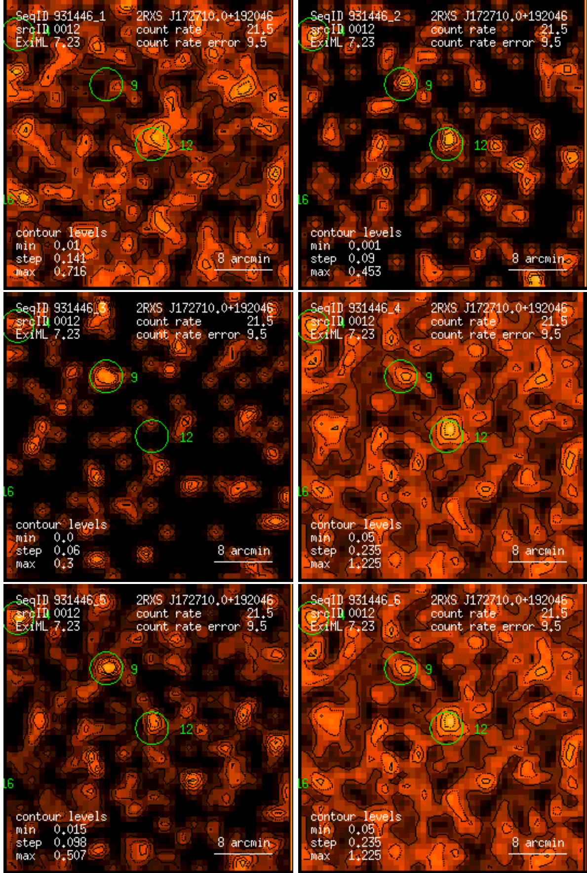
Figure 12: RASS 931446: detection 0012: band rate images, Gaussian filter: (1) PSPC channels 11 – 41, (2) 52 – 90, (3) 91 – 201, (4) 11 – 235, (5) 52 – 201, (6) 11 – 201. Broad band rates in counts/ks. Band rate contour levels in counts/ks/arcmin 2 .
