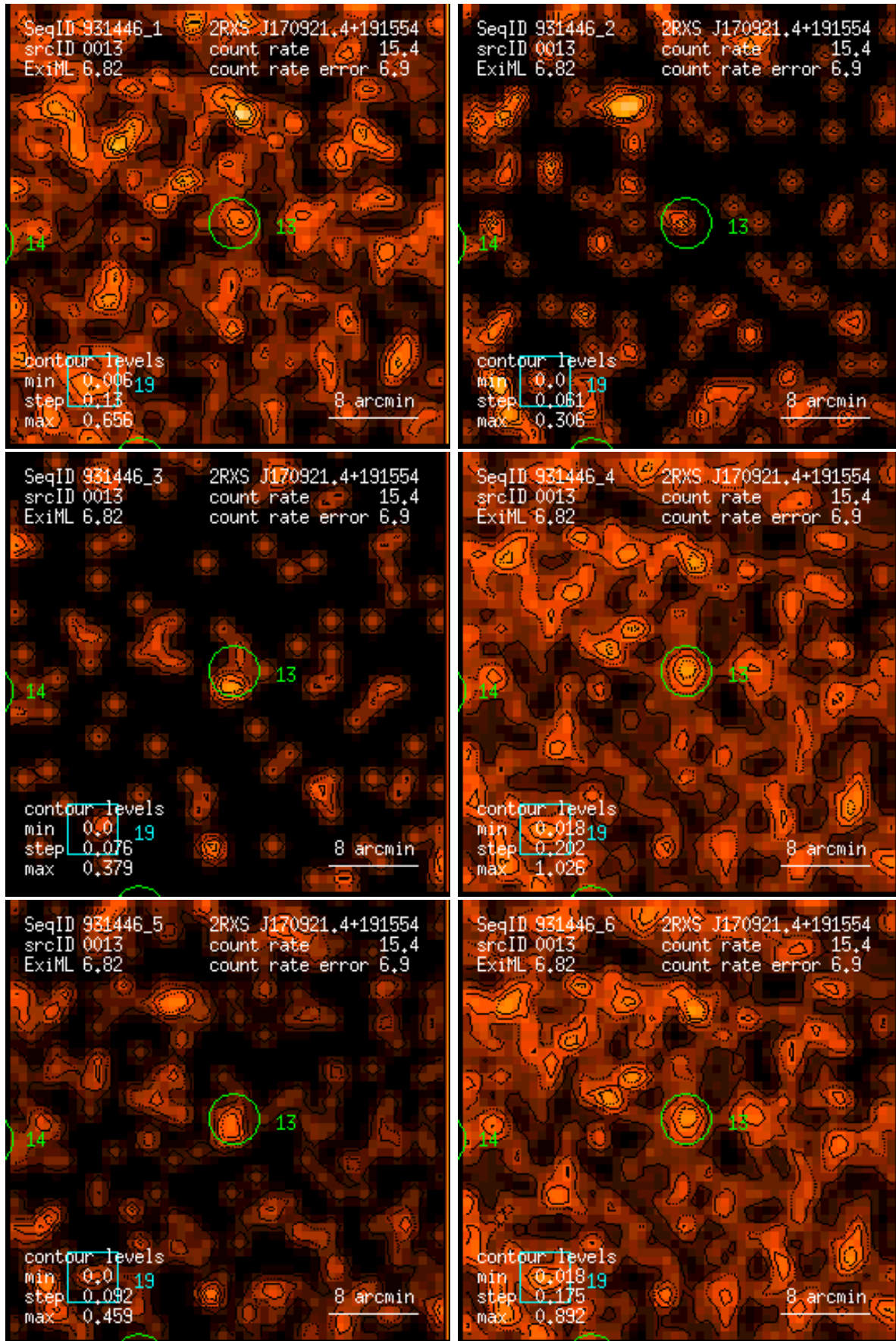
Figure 13: RASS 931446: detection 0013: band rate images, Gaussian filter: (1) PSPC channels 11 – 41, (2) 52 – 90, (3) 91 – 201, (4) 11 – 235, (5) 52 – 201, (6) 11 – 201. Broad band rates in counts/ks. Band rate contour levels in counts/ks/arcmin 2 .
