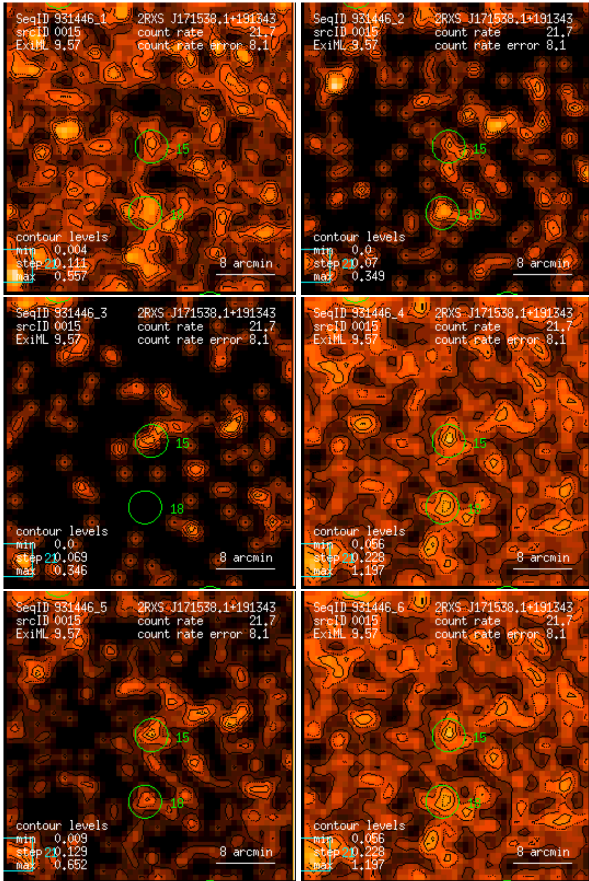
Figure 15: RASS 931446: detection 0015: band rate images, Gaussian filter: (1) PSPC channels 11 – 41, (2) 52 – 90, (3) 91 – 201, (4) 11 – 235, (5) 52 – 201, (6) 11 – 201. Broad band rates in counts/ks. Band rate contour levels in counts/ks/arcmin 2 .
