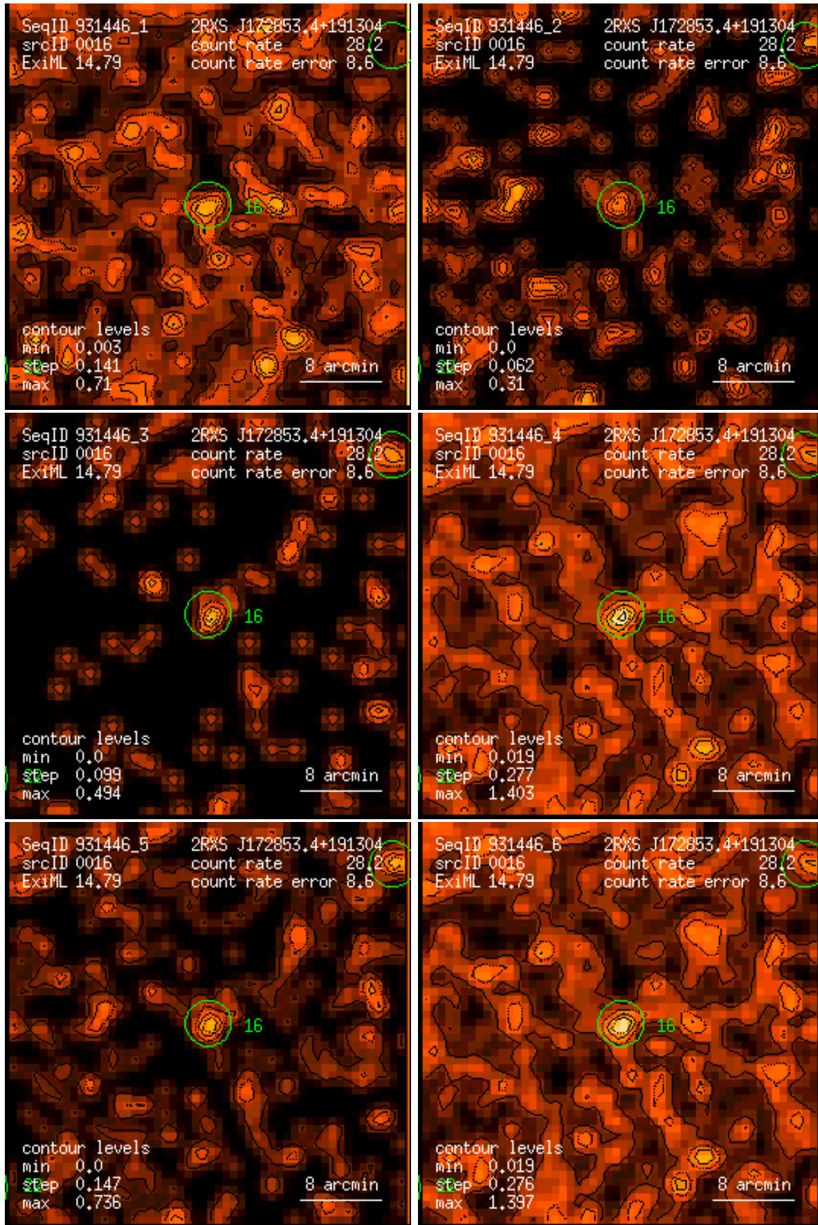
Figure 16: RASS 931446: detection 0016: band rate images, Gaussian filter: (1) PSPC channels 11 – 41, (2) 52 – 90, (3) 91 – 201, (4) 11 – 235, (5) 52 – 201, (6) 11 – 201. Broad band rates in counts/ks. Band rate contour levels in counts/ks/arcmin 2 .
