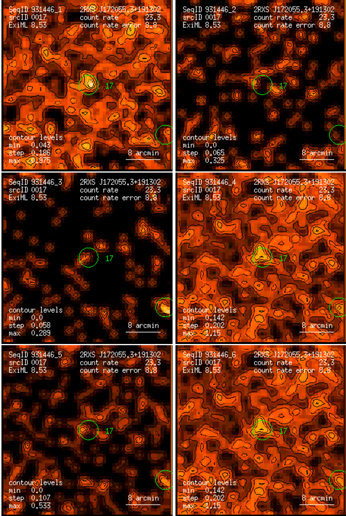
Figure 17: RASS 931446: detection 0017: band rate images, Gaussian filter: (1) PSPC channels 11 – 41, (2) 52 – 90, (3) 91 – 201, (4) 11 – 235, (5) 52 – 201, (6) 11 – 201. Broad band rates in counts/ks. Band rate contour levels in counts/ks/arcmin 2 .
