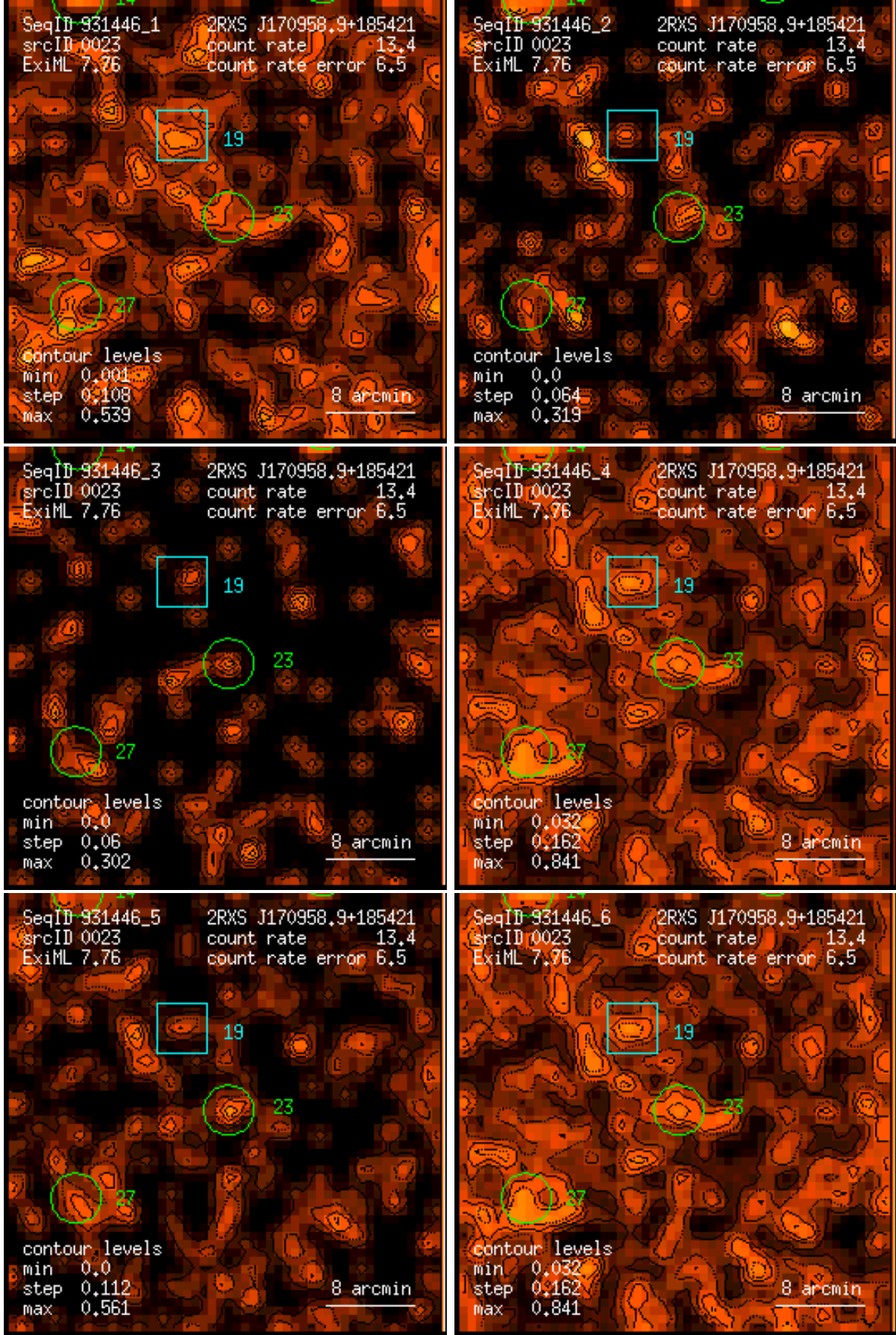
Figure 23: RASS 931446: detection 0023: band rate images, Gaussian filter: (1) PSPC channels 11 – 41, (2) 52 – 90, (3) 91 – 201, (4) 11 – 235, (5) 52 – 201, (6) 11 – 201. Broad band rates in counts/ks. Band rate contour levels in counts/ks/arcmin 2 .
