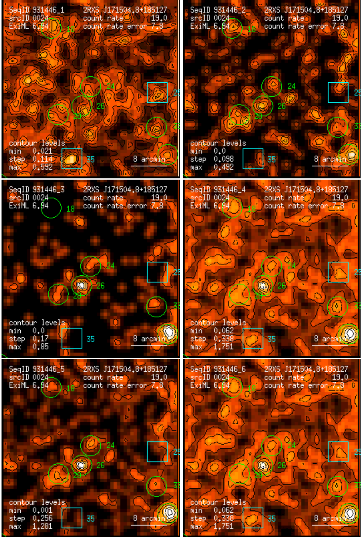
Figure 24: RASS 931446: detection 0024: band rate images, Gaussian filter: (1) PSPC channels 11 – 41, (2) 52 – 90, (3) 91 – 201, (4) 11 – 235, (5) 52 – 201, (6) 11 – 201. Broad band rates in counts/ks. Band rate contour levels in counts/ks/arcmin 2 .
