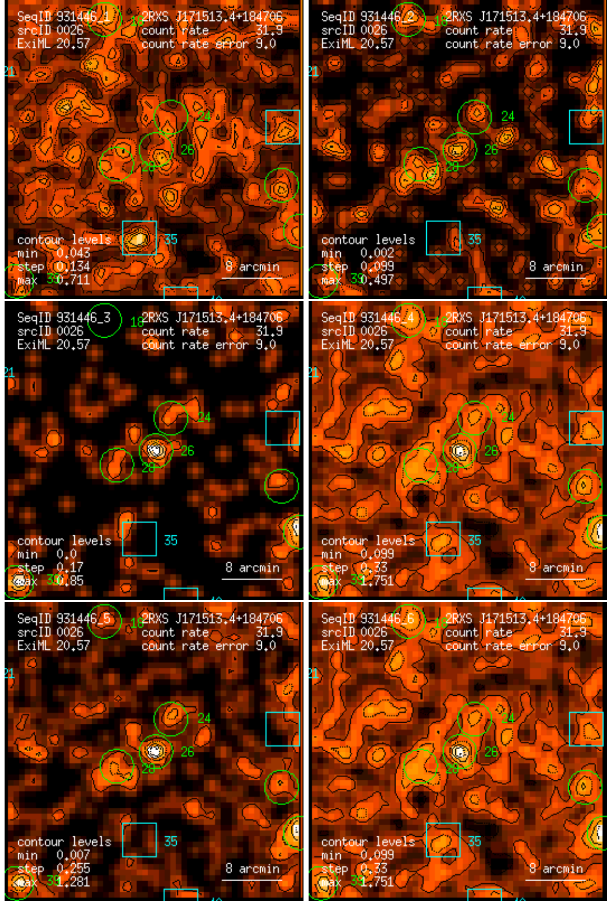
Figure 26: RASS 931446: detection 0026: band rate images, Gaussian filter: (1) PSPC channels 11 – 41, (2) 52 – 90, (3) 91 – 201, (4) 11 – 235, (5) 52 – 201, (6) 11 – 201. Broad band rates in counts/ks. Band rate contour levels in counts/ks/arcmin 2 .
