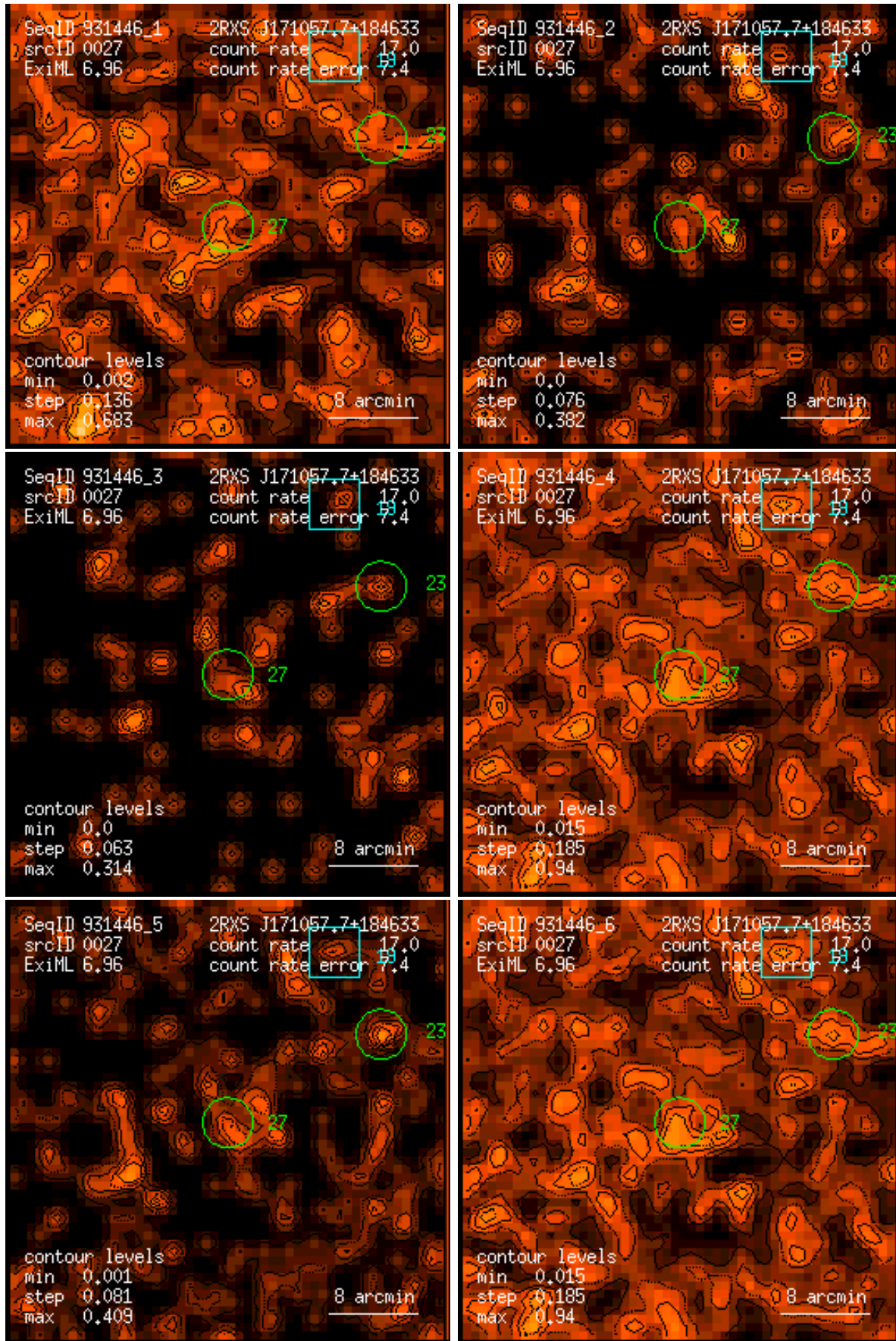
Figure 27: RASS 931446: detection 0027: band rate images, Gaussian filter: (1) PSPC channels 11 – 41, (2) 52 – 90, (3) 91 – 201, (4) 11 – 235, (5) 52 – 201, (6) 11 – 201. Broad band rates in counts/ks. Band rate contour levels in counts/ks/arcmin 2 .
