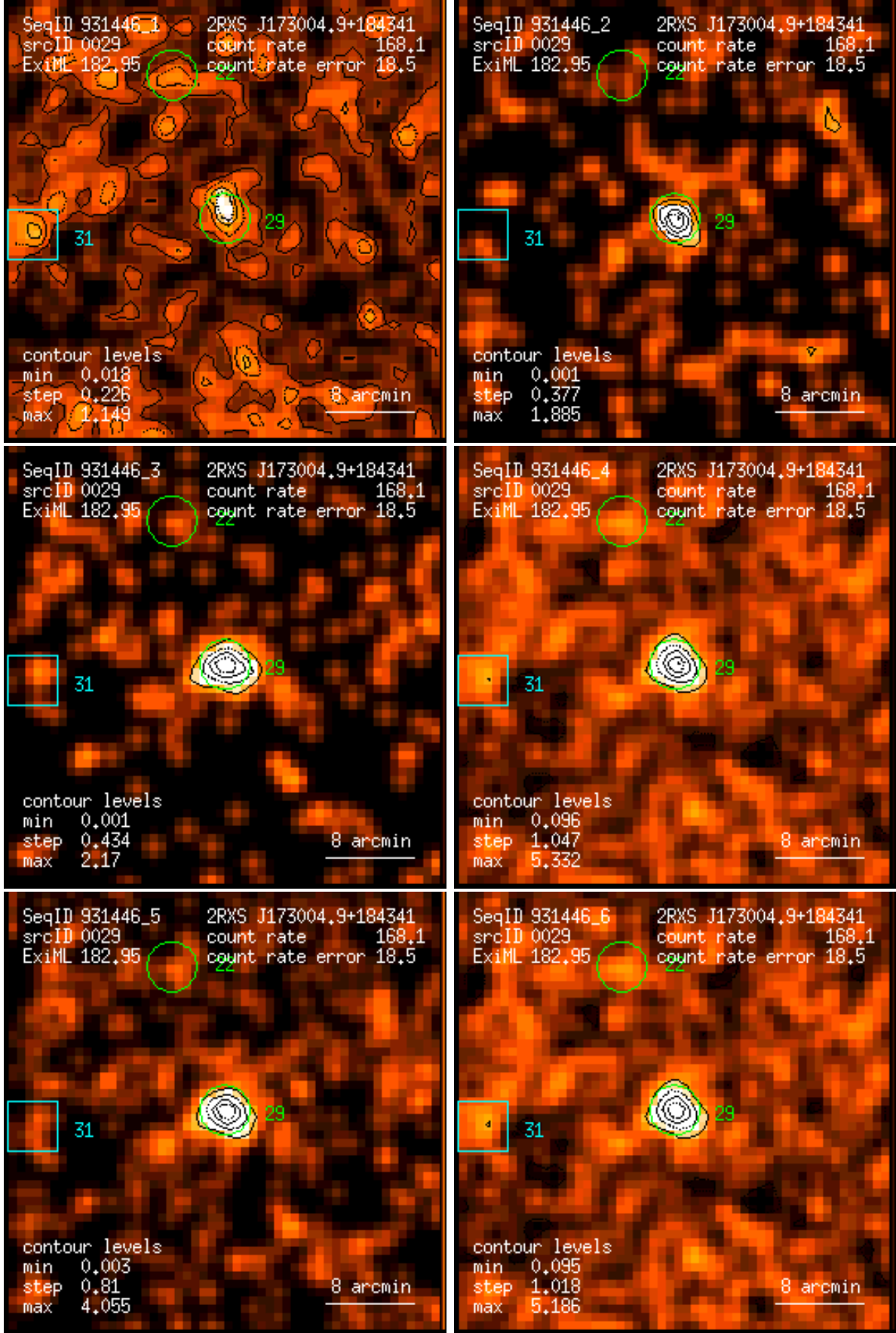
Figure 29: RASS 931446: detection 0029: band rate images, Gaussian filter: (1) PSPC channels 11 – 41, (2) 52 – 90, (3) 91 – 201, (4) 11 – 235, (5) 52 – 201, (6) 11 – 201. Broad band rates in counts/ks. Band rate contour levels in counts/ks/arcmin 2 .
