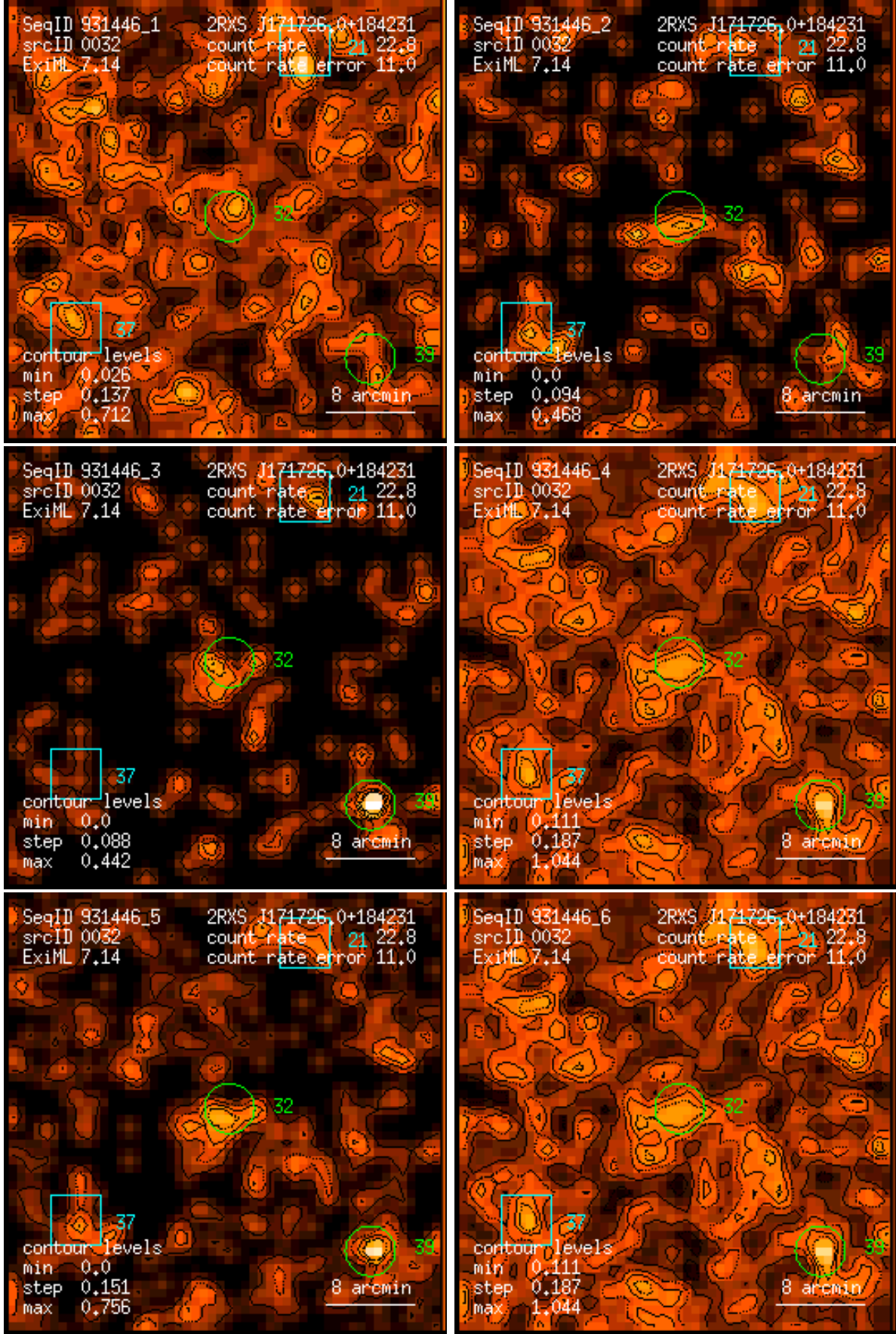
Figure 32: RASS 931446: detection 0032: band rate images, Gaussian filter: (1) PSPC channels 11 – 41, (2) 52 – 90, (3) 91 – 201, (4) 11 – 235, (5) 52 – 201, (6) 11 – 201. Broad band rates in counts/ks. Band rate contour levels in counts/ks/arcmin 2 .
