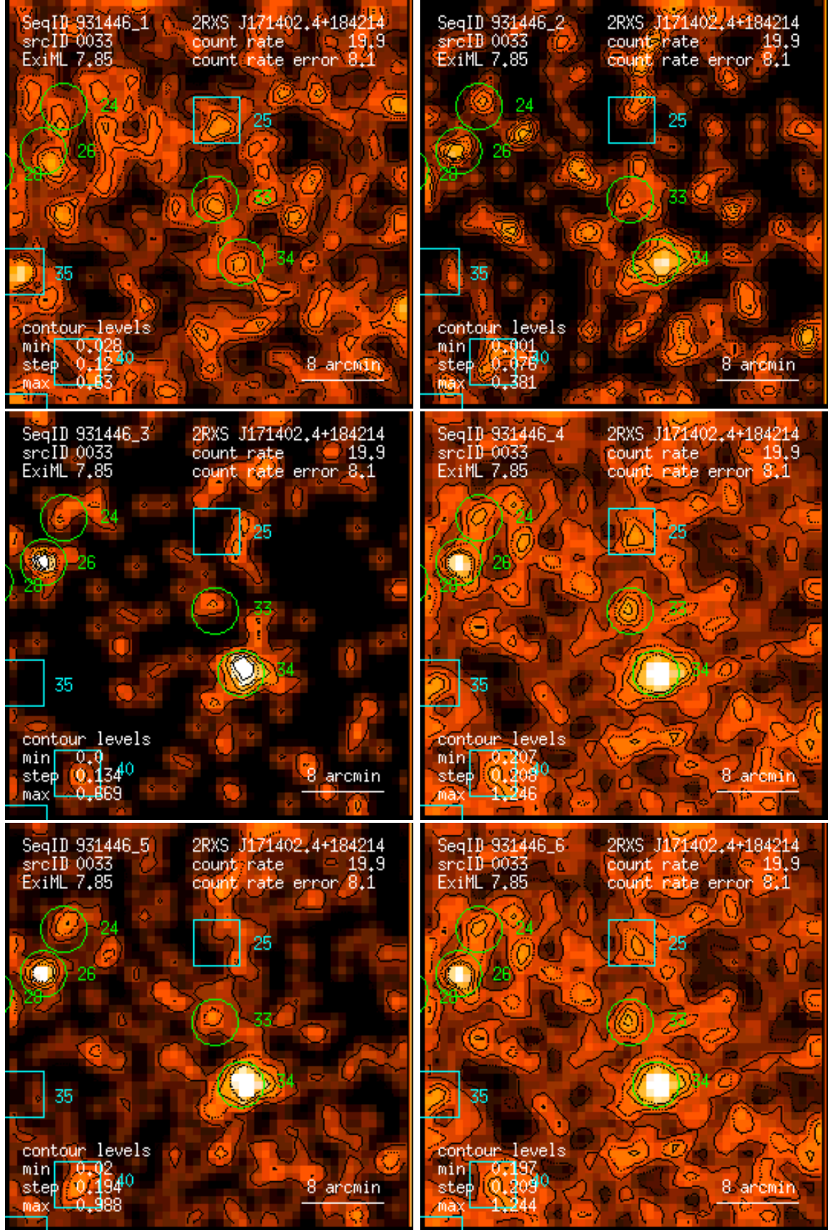
Figure 33: RASS 931446: detection 0033: band rate images, Gaussian filter: (1) PSPC channels 11 – 41, (2) 52 – 90, (3) 91 – 201, (4) 11 – 235, (5) 52 – 201, (6) 11 – 201. Broad band rates in counts/ks. Band rate contour levels in counts/ks/arcmin 2 .
