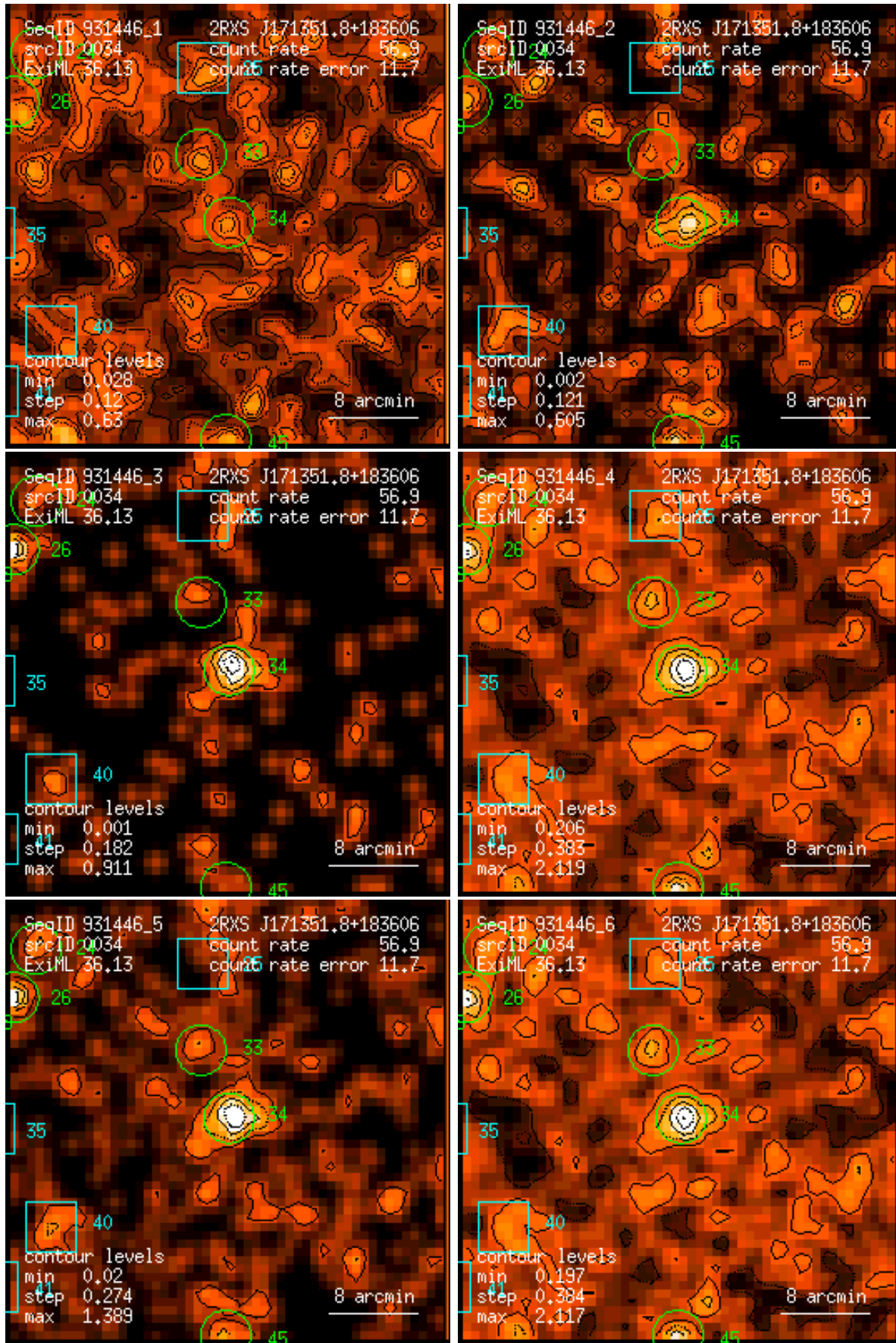
Figure 34: RASS 931446: detection 0034: band rate images, Gaussian filter: (1) PSPC channels 11 – 41, (2) 52 – 90, (3) 91 – 201, (4) 11 – 235, (5) 52 – 201, (6) 11 – 201. Broad band rates in counts/ks. Band rate contour levels in counts/ks/arcmin 2 .
