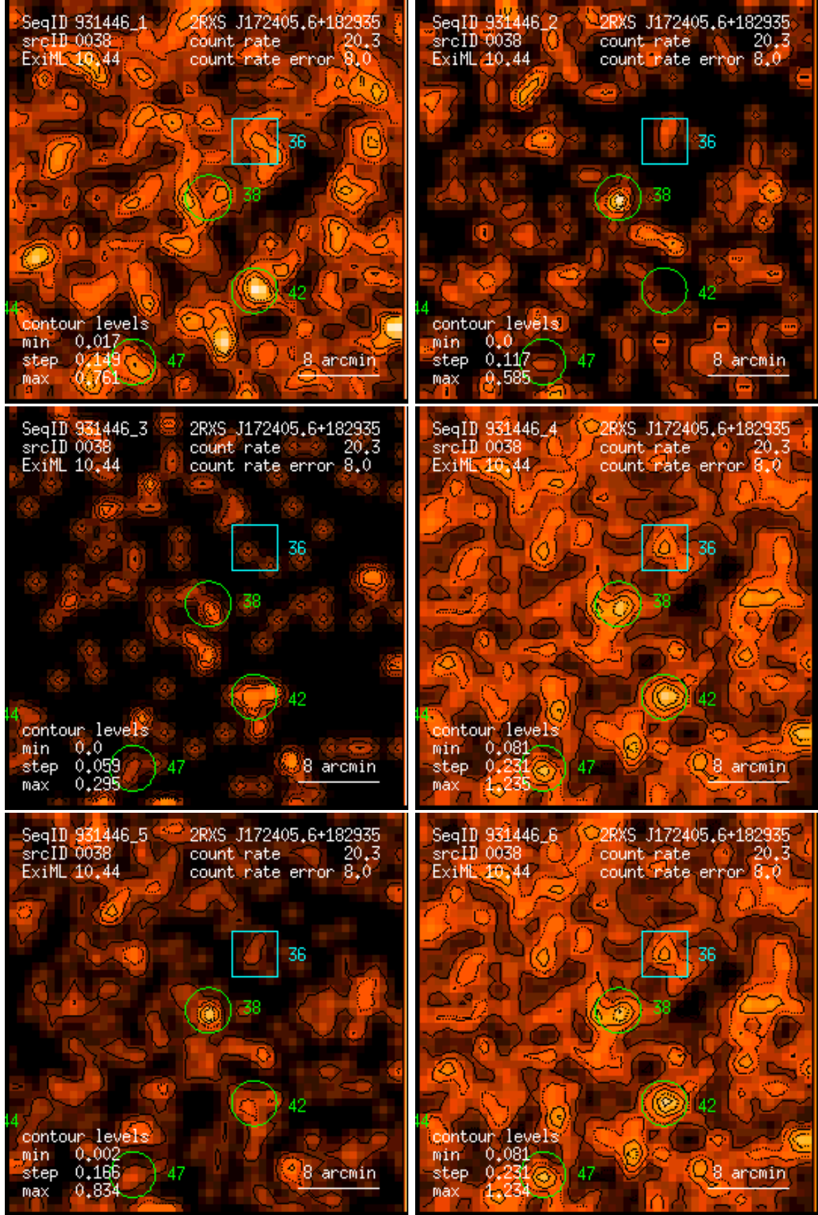
Figure 38: RASS 931446: detection 0038: band rate images, Gaussian filter: (1) PSPC channels 11 – 41, (2) 52 – 90, (3) 91 – 201, (4) 11 – 235, (5) 52 – 201, (6) 11 – 201. Broad band rates in counts/ks. Band rate contour levels in counts/ks/arcmin 2 .
