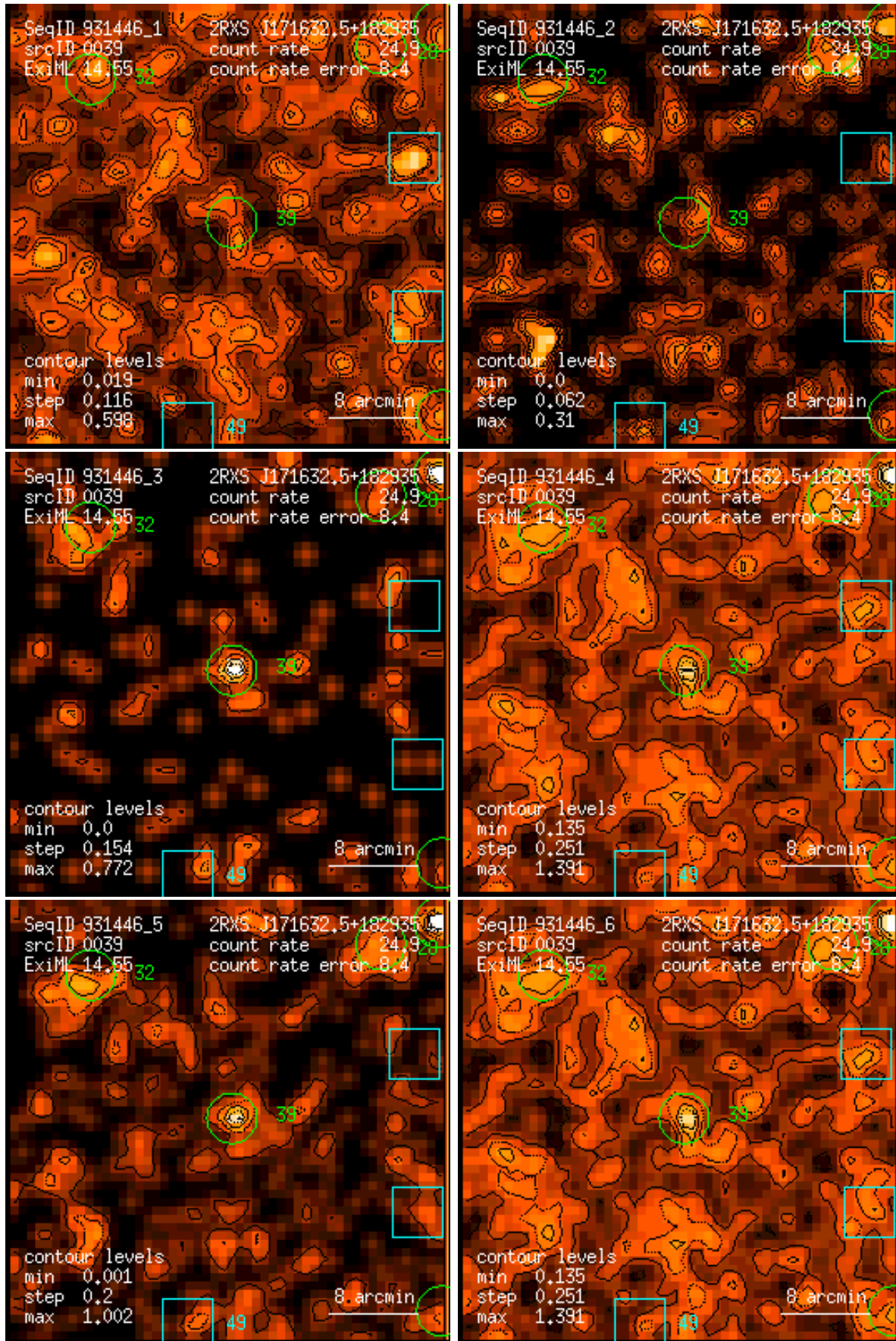
Figure 39: RASS 931446: detection 0039: band rate images, Gaussian filter: (1) PSPC channels 11 – 41, (2) 52 – 90, (3) 91 – 201, (4) 11 – 235, (5) 52 – 201, (6) 11 – 201. Broad band rates in counts/ks. Band rate contour levels in counts/ks/arcmin 2 .
