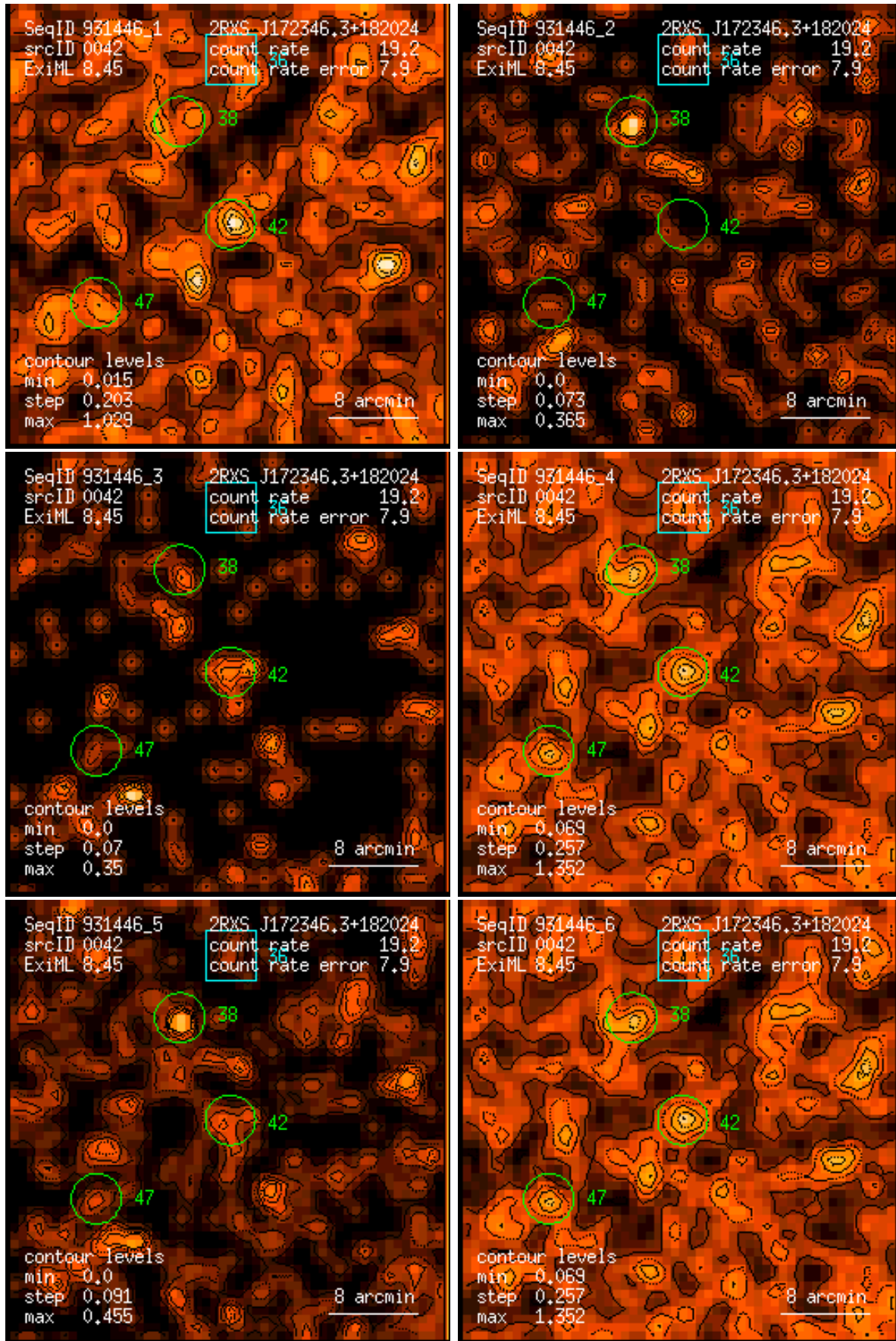
Figure 42: RASS 931446: detection 0042: band rate images, Gaussian filter: (1) PSPC channels 11 – 41, (2) 52 – 90, (3) 91 – 201, (4) 11 – 235, (5) 52 – 201, (6) 11 – 201. Broad band rates in counts/ks. Band rate contour levels in counts/ks/arcmin 2 .
