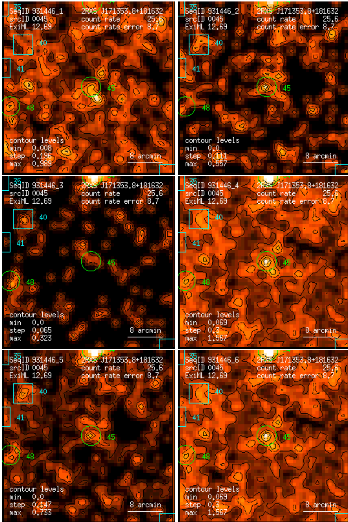
Figure 45: RASS 931446: detection 0045: band rate images, Gaussian filter: (1) PSPC channels 11 – 41, (2) 52 – 90, (3) 91 – 201, (4) 11 – 235, (5) 52 – 201, (6) 11 – 201. Broad band rates in counts/ks. Band rate contour levels in counts/ks/arcmin 2 .
