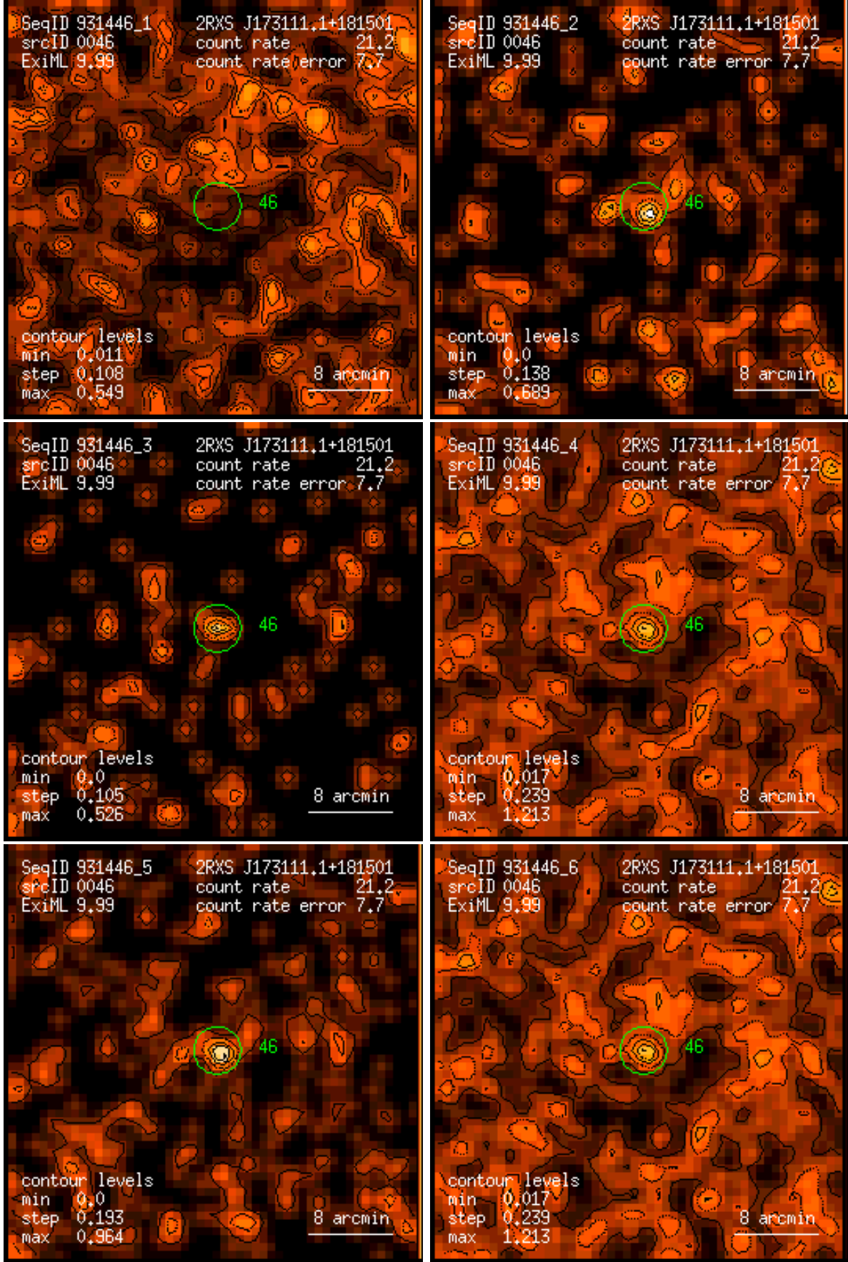
Figure 46: RASS 931446: detection 0046: band rate images, Gaussian filter: (1) PSPC channels 11 – 41, (2) 52 – 90, (3) 91 – 201, (4) 11 – 235, (5) 52 – 201, (6) 11 – 201. Broad band rates in counts/ks. Band rate contour levels in counts/ks/arcmin 2 .
