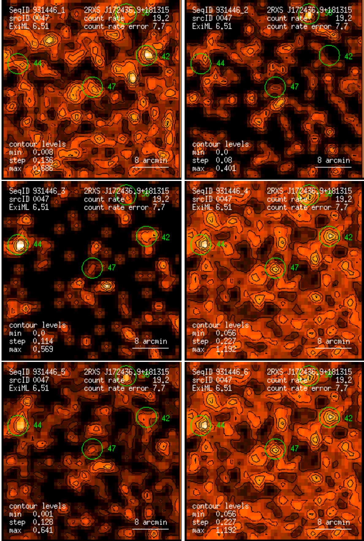
Figure 47: RASS 931446: detection 0047: band rate images, Gaussian filter: (1) PSPC channels 11 – 41, (2) 52 – 90, (3) 91 – 201, (4) 11 – 235, (5) 52 – 201, (6) 11 – 201. Broad band rates in counts/ks. Band rate contour levels in counts/ks/arcmin 2 .
