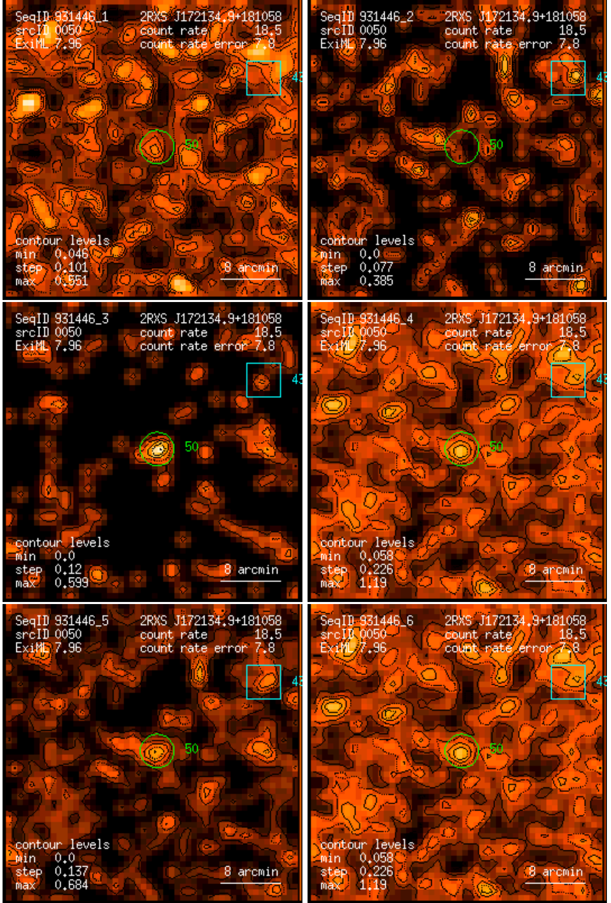
Figure 50: RASS 931446: detection 0050: band rate images, Gaussian filter: (1) PSPC channels 11 – 41, (2) 52 – 90, (3) 91 – 201, (4) 11 – 235, (5) 52 – 201, (6) 11 – 201. Broad band rates in counts/ks. Band rate contour levels in counts/ks/arcmin 2 .
