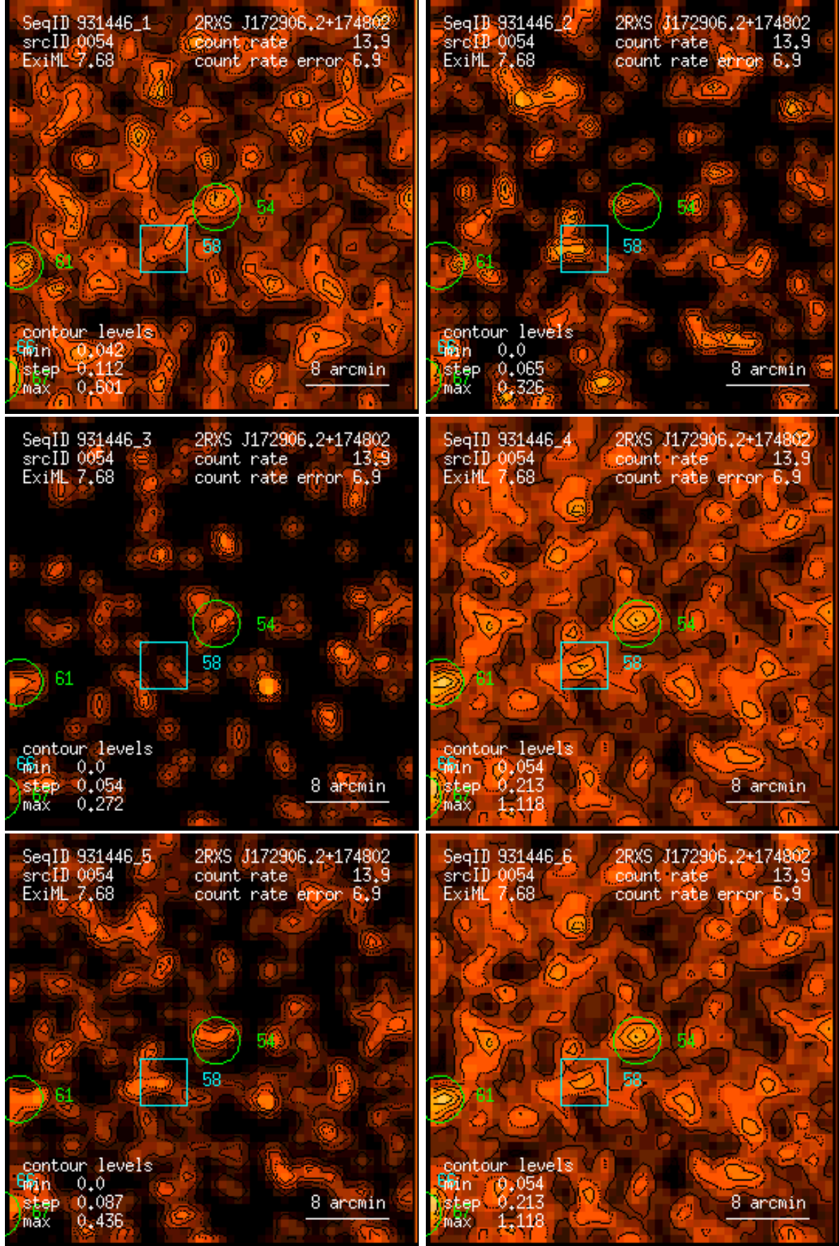
Figure 54: RASS 931446: detection 0054: band rate images, Gaussian filter: (1) PSPC channels 11 – 41, (2) 52 – 90, (3) 91 – 201, (4) 11 – 235, (5) 52 – 201, (6) 11 – 201. Broad band rates in counts/ks. Band rate contour levels in counts/ks/arcmin 2 .
