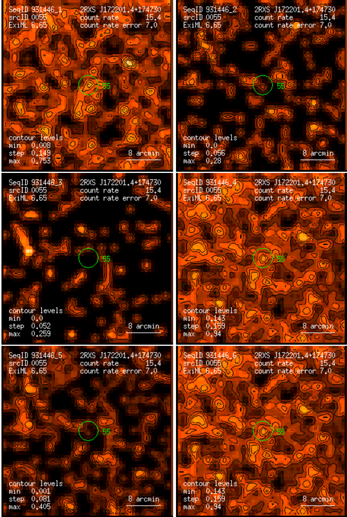
Figure 55: RASS 931446: detection 0055: band rate images, Gaussian filter: (1) PSPC channels 11 – 41, (2) 52 – 90, (3) 91 – 201, (4) 11 – 235, (5) 52 – 201, (6) 11 – 201. Broad band rates in counts/ks. Band rate contour levels in counts/ks/arcmin 2 .
