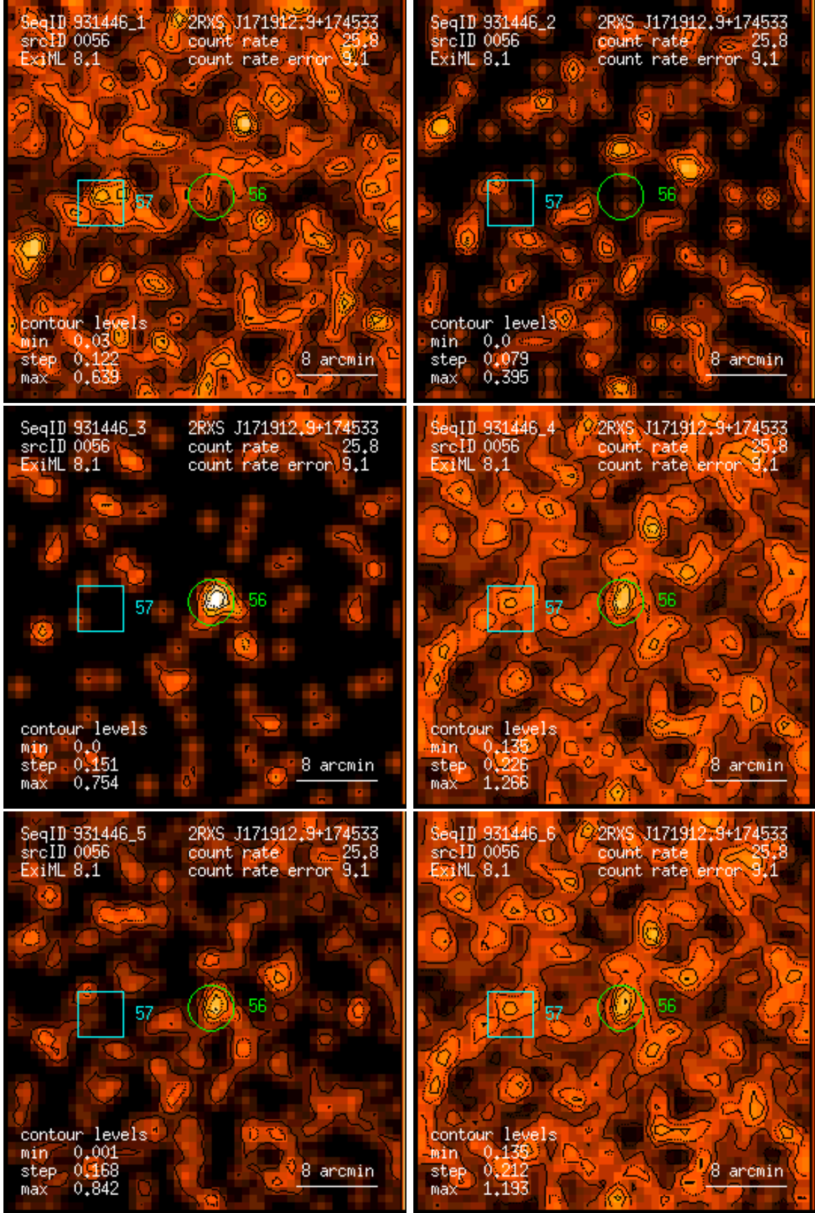
Figure 56: RASS 931446: detection 0056: band rate images, Gaussian filter: (1) PSPC channels 11 – 41, (2) 52 – 90, (3) 91 – 201, (4) 11 – 235, (5) 52 – 201, (6) 11 – 201. Broad band rates in counts/ks. Band rate contour levels in counts/ks/arcmin 2 .
