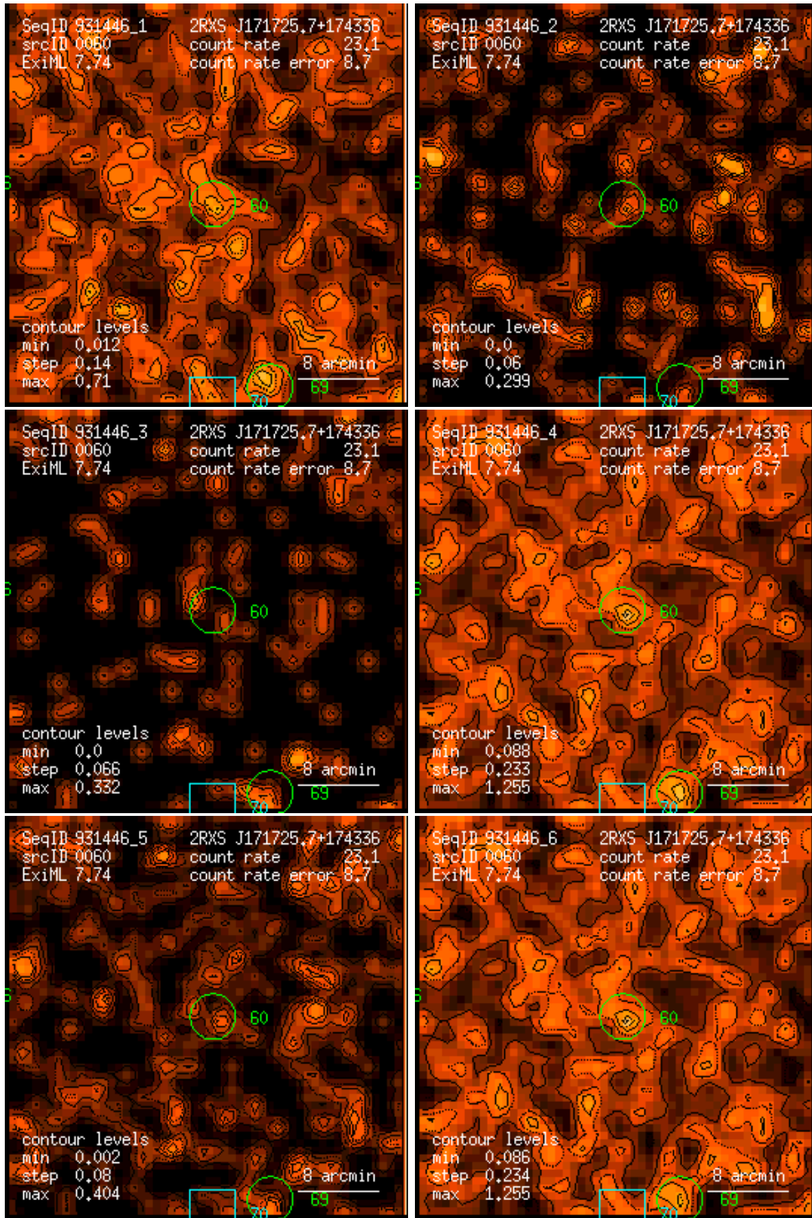
Figure 60: RASS 931446: detection 0060: band rate images, Gaussian filter: (1) PSPC channels 11 – 41, (2) 52 – 90, (3) 91 – 201, (4) 11 – 235, (5) 52 – 201, (6) 11 – 201. Broad band rates in counts/ks. Band rate contour levels in counts/ks/arcmin 2 .
