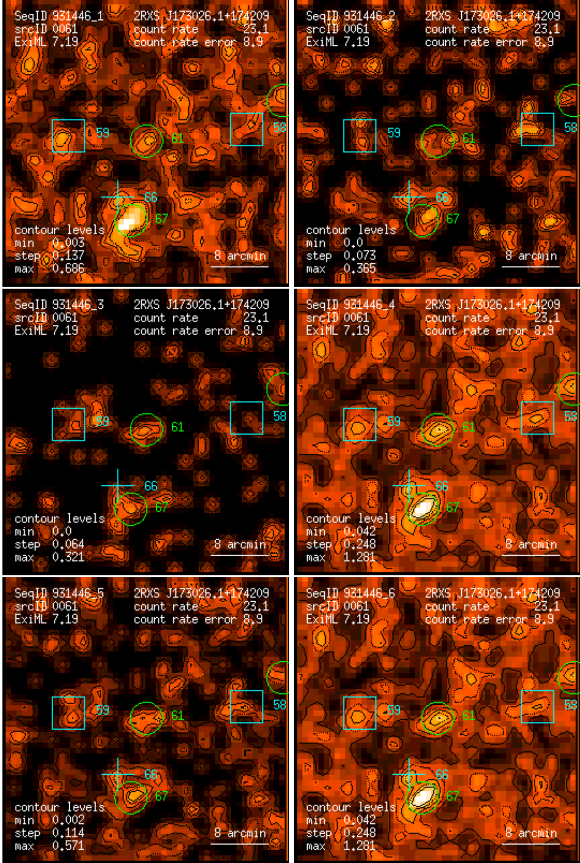
Figure 61: RASS 931446: detection 0061: band rate images, Gaussian filter: (1) PSPC channels 11 – 41, (2) 52 – 90, (3) 91 – 201, (4) 11 – 235, (5) 52 – 201, (6) 11 – 201. Broad band rates in counts/ks. Band rate contour levels in counts/ks/arcmin 2 .
