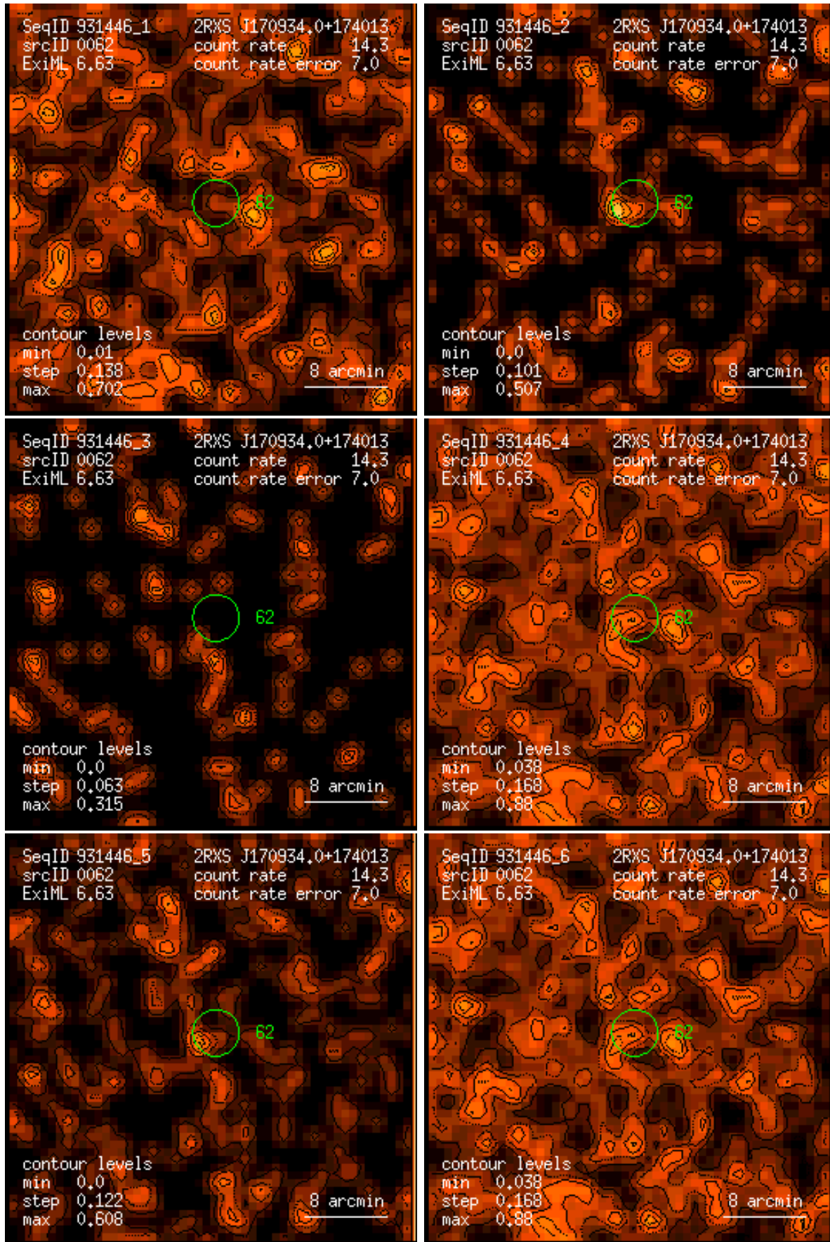
Figure 62: RASS 931446: detection 0062: band rate images, Gaussian filter: (1) PSPC channels 11 – 41, (2) 52 – 90, (3) 91 – 201, (4) 11 – 235, (5) 52 – 201, (6) 11 – 201. Broad band rates in counts/ks. Band rate contour levels in counts/ks/arcmin 2 .
