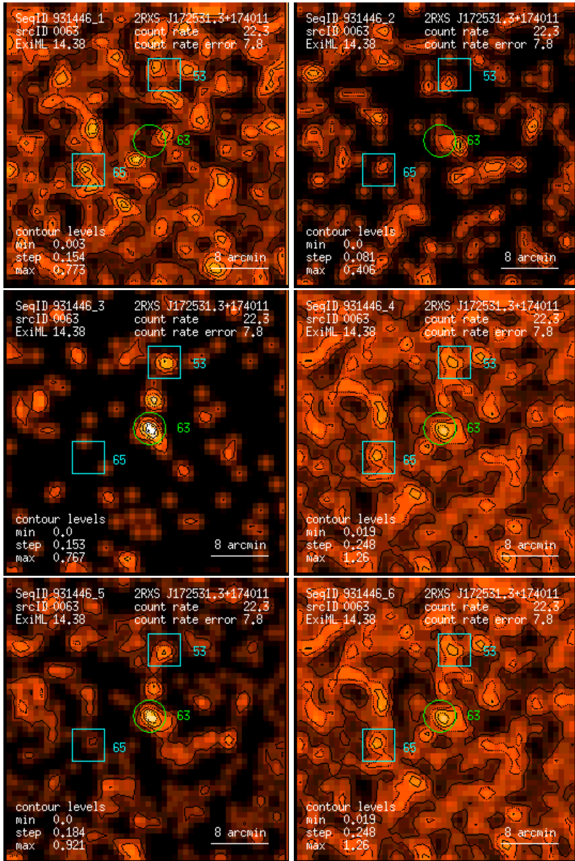
Figure 63: RASS 931446: detection 0063: band rate images, Gaussian filter: (1) PSPC channels 11 – 41, (2) 52 – 90, (3) 91 – 201, (4) 11 – 235, (5) 52 – 201, (6) 11 – 201. Broad band rates in counts/ks. Band rate contour levels in counts/ks/arcmin 2 .
