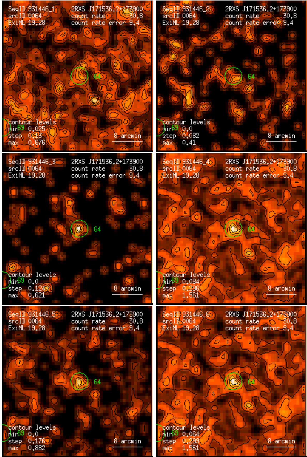
Figure 64: RASS 931446: detection 0064: band rate images, Gaussian filter: (1) PSPC channels 11 – 41, (2) 52 – 90, (3) 91 – 201, (4) 11 – 235, (5) 52 – 201, (6) 11 – 201. Broad band rates in counts/ks. Band rate contour levels in counts/ks/arcmin 2 .
